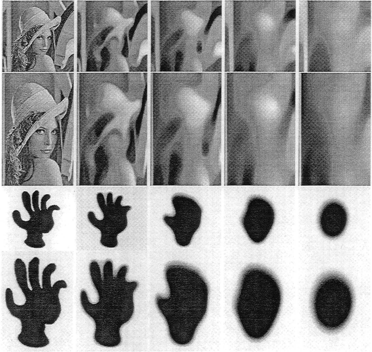
Figure 4: The evolution (left to right) of two images: The original planar flow and its corresponding \kappa_g flow of the planar image mapped onto a cylinder. The original image x -axis is scaled to the cylinder diameter size. The results show the invariance to bending of the original image plane onto a cylinder.
