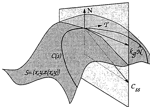
Figure 1: The geometry of the geodesic curvature vector, \kappa_g \hat{\mathcal{N}} .
