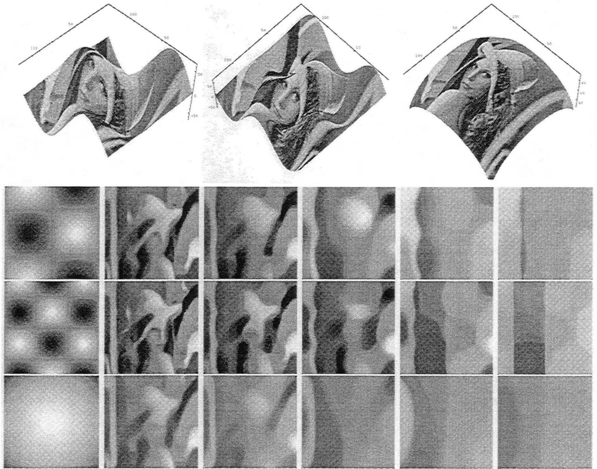
Figure 5: The evolution (left to right) of Lenna image, this time projected onto three surfaces (at the top). The surfaces are also presented to the left of the evolution sequence: Gray level corresponds to the height.
