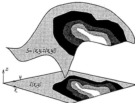
Figure 2: The image I(x, y) is painted on the parameterized surface \mathcal{S} = (x, y, z(x, y)) . I.e. the surface point (x, y, z(x, y)) has the gray level I(x, y) .
