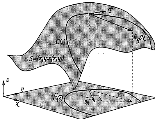
Figure 3: The geometry of the geodesic curvature vector projection.
