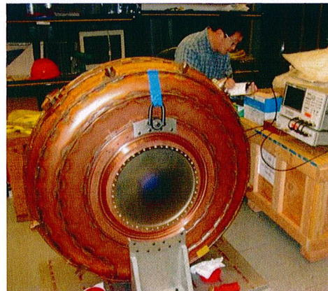
Figure 5: MICE RF cavity measurements with curved beryllium windows at LBNL.
