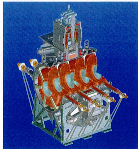
Figure 2: A cut-away view of the RFCC module of the MICE cooling channel: four 201-MHz normal conducting RF cavities with thin beryllium windows are installed in a vacuum vessel, surrounded by the CC magnet that is cooled by three cryocoolers.
