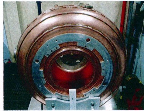
Figure 8: The first MICE cavity electro-polished at LBNL in May 2012.
