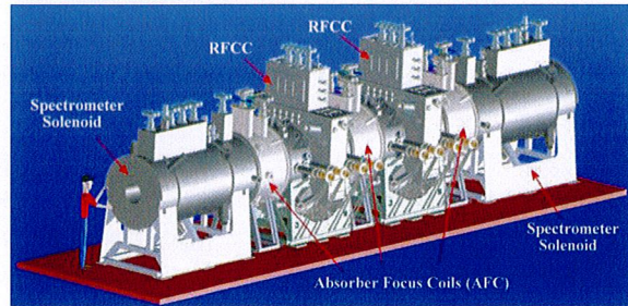
Figure 1: A schematic layout (3-dimensional CAD model) of the MICE experiment with major components.
