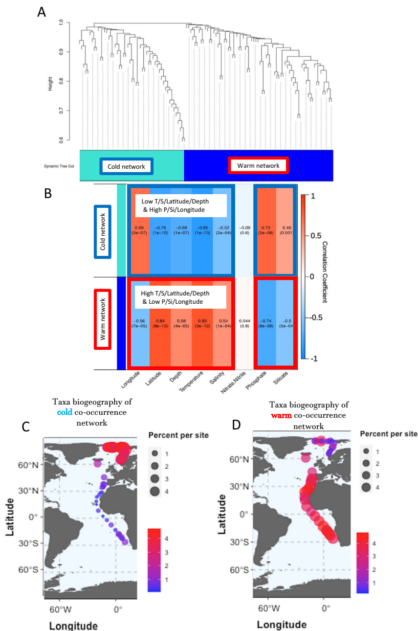
Fig. 4 Co-occurrence networks of 16 and 18S rDNAs, their biodiversity and biogeographical mapping of the node-specific abundance for each taxonomic network across all stations from pole to pole. On the log 10 transformed abundances of 18S rDNA species level and 16S rDNA genus level, two networks were found: A cold ( n = 51 ) and warm ( n = 70 ). A list of species names and class names of the species can be found in the Supplementary Table 2. B Co-occurrence analysis of 18S rDNA species level and 16S rDNA genus level, two networks were found, a turquoise (cold) and blue (warm). Correlation heatmap between the networks and environmental parameters. The colours correspond to the correlation values, red is positively correlated and blue is negatively correlated. The values in each of the squares correspond to the assigned Pearson correlation coefficient value on top and p -value in brackets below. C Taxa biogeography of cold 16/18S co-occurrence network. D Taxa biogeography of warm 16/18S co-occurrence network. Abundance is given in percentage contribution to the total sequence pool per site with increasing contribution from small to large circles and from blue to red.
