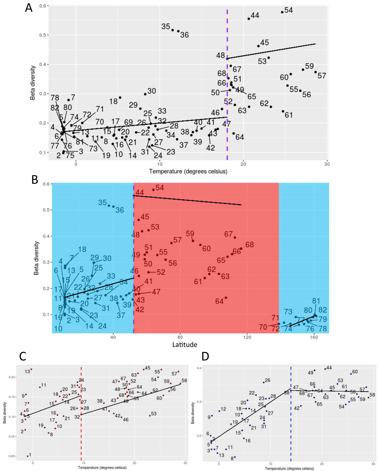
Fig. 5 Beta diversity break-point analyses. A, B Represent breakpoints of protein families as part of the metatranscriptome dataset. C, D Represent breakpoints of the 18S rDNA and 16S rDNA datasets. The numbers correspond to sample locations as shown in Fig. 1A. The y-axis represents beta diversity across all stations. The x-axis in A, C and D represents temperature and in B represents latitude. The horizontal lines indicate the breakpoints in beta diversity. For the Pfam protein families dataset in ( A ), the breakpoint is at 18.06 °C with a p -value of 3.741e-10 . In B the breakpoint is at 52.167 degrees altered latitude (37.833 degrees latitude) with a p -value of 2.225e-07 . For the 16S rDNA dataset in ( C ), the breakpoint is at 9.49 °C with a p -value of 1.413e-4 . For the 18S rDNA dataset in ( D ), the breakpoint is at 13.96 °C with a p -value of 8.407e-11 .
