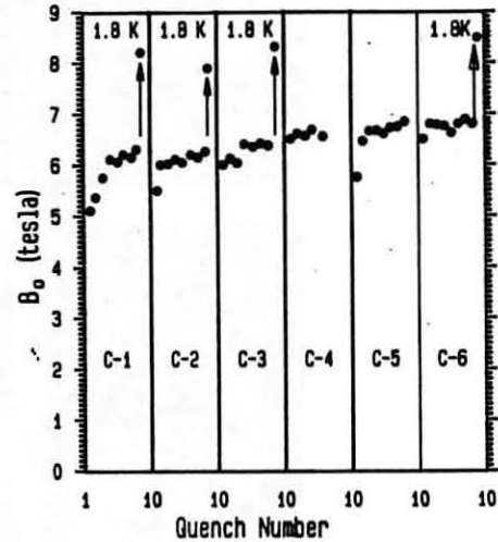
Fig. 8 Training behavior of the first six 1-m LBL SSC dipole models at 4.4K. C-1,2 have 25 mm Al collars; C-2 has 15 mm machined collars, C-4,5,6 have 15 mm stamped collars and improved cable. Critical field achieved at 1.8K is shown.
