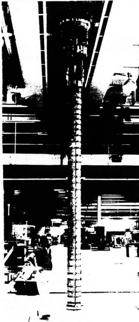
Fig. 10 4.5 m BNL model with a circular laminated iron yoke ready for testing in a vertical cryostat.
