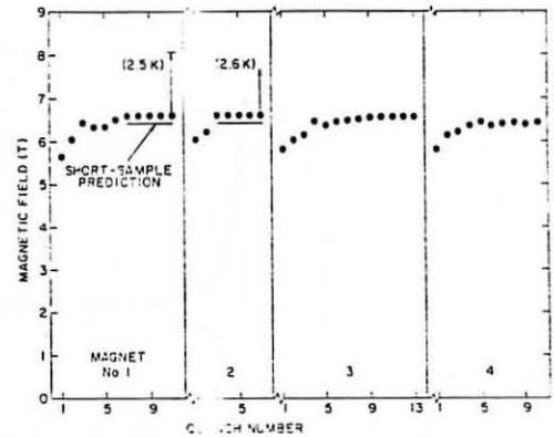
Fig. 11 Magnetic field at quench of four 4.5 m BNL SSC dipole models at 4.5K.
