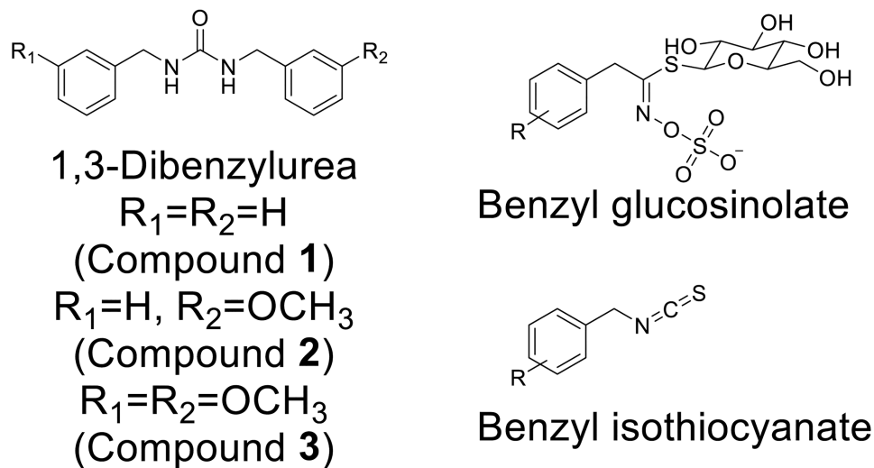
Fig 1. Chemical structures of 1, 3-dibenzylurea, benzyl glucosinolate and isothiocyanate.
