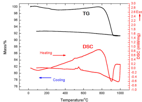
Figure 5. TG-DSC of K_8Al_8Si_{38} measured from 25 °C to 1000 °C heating and then cooling under flowing argon. Reprinted with permission from Sui, F.; Kauzlarich, S.M. Tuning Thermoelectric Properties of Type I Clathrate K_{8-x}Ba_xAl_{8+x}Si_{38-x} through Barium Substitution. Chem. Mater. 2016 , 28 , 3099–3107 [37]. Copyright (2016) American Chemical Society.
