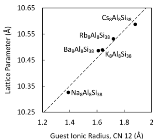
Figure 3. Lattice parameter vs. guest ionic radii for coordination number (CN) = 12 for A_8Al_8Si_{38} . Reprinted with permission from Dong, Y.K.; Chai, P.; Beekman, M.; Zeng, X.Y.; Tritt, T.M.; Nolas, G.S. Precursor Routes to Complex Ternary Intermetallics: Single-Crystal and Microcrystalline Preparation of Clathrate-I Na_8Al_8Si_{38} from NaSi plus NaAlSi. Inorg. Chem. 2015 , 54 , 5316–5321 [9]. Copyright (2015) American Chemical Society.
