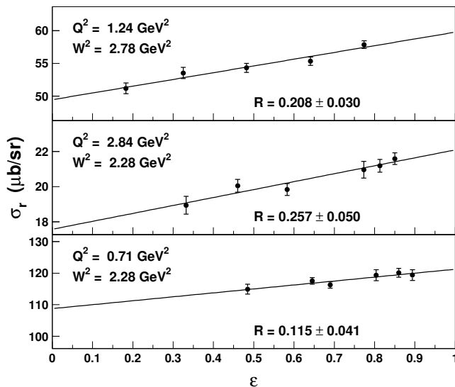
FIG. 1. Representative Rosenbluth plots for the kinematics indicated.
