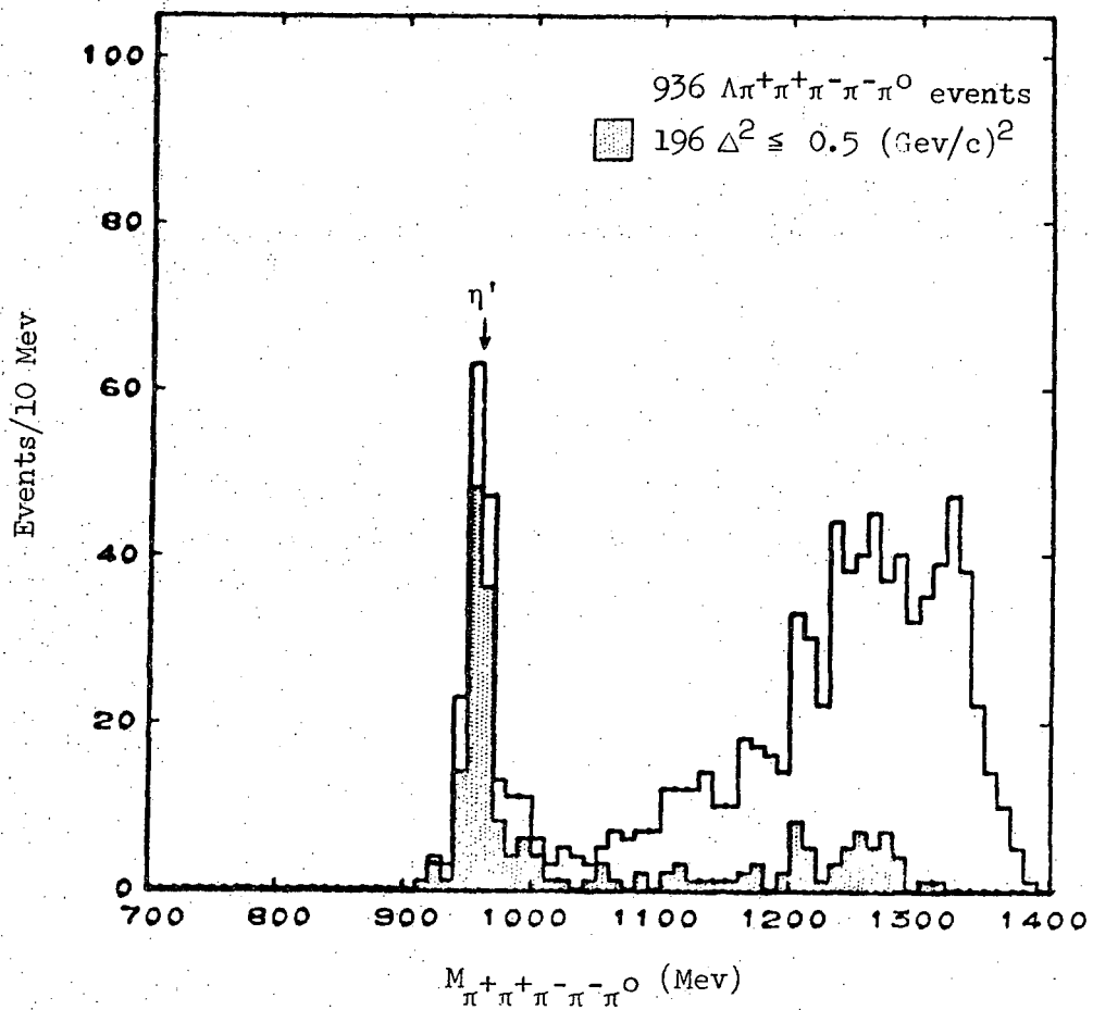
Figure 3. The M_{\pi^+\pi^+\pi^-\pi^-\pi^0} mass spectrum for events fitting the reaction K^-p \rightarrow \Lambda \pi^+ \pi^+ \pi^- \pi^- \pi^0 . The shaded events are those with \Delta^2 \leq 0.5 \text{ (GeV/c)}^2 .
