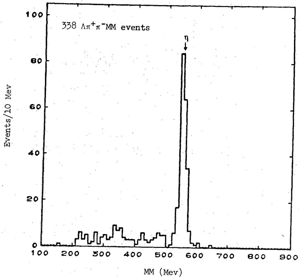
Figure 10. The projection of Figure 9 onto the MM axis for \Lambda\pi^+\pi^-MM events with 950 \leq M_{\pi^+\pi^-MM} \leq 970 Mev.
