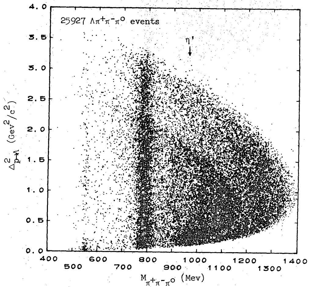
Figure 15. The Chew-Low plot for the \Lambda\pi^+\pi^-\pi^0 events of Figure 14.
