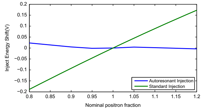
Fig. 23. Energy shift for standard and autoresonant injection schemes. The abscissa is fractional variation from a nominal N_0 = 2 \times 10^6 positrons. The energy shift shown is \Delta U_i(N_0) - \Delta U_i for the standard injection and \Delta U_f - \Delta U_f(N_0) for autoresonant injection. Antiprotons with negative energy shifts in the standard injection scheme do not pass through the positrons.
