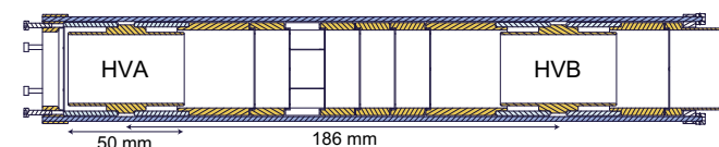
Fig. 4. Axial section of the catching trap electrodes with the two high voltage electrodes used for catching the energetic antiprotons highlighted. The six-fold segmented electrode is apparent.
