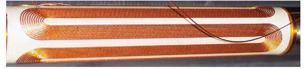
Fig. 9. First layer of the octupole [20].
