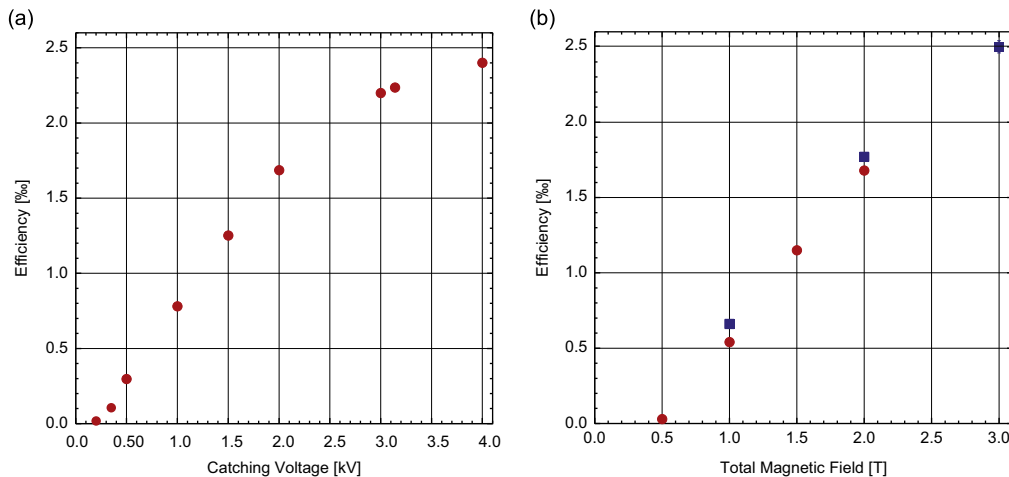
Fig. 17. Antiproton catching efficiencies. (a) Efficiency as a function of HVA gate voltage for V_{HVB} = 4 kV in a 3 T field and (b) efficiency as a function of magnetic field strength for the high voltages set to V_{HV} = 4 kV. ● inner solenoid only, ■ inner solenoid plus 1 T from external solenoid.
