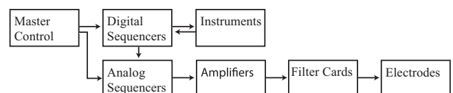
Fig. 15. Block diagram of the sequencer and amplifier setup.
