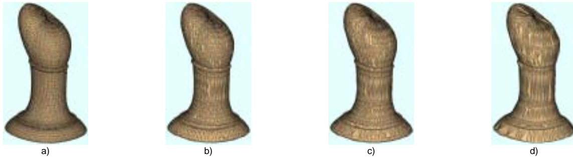
Figure 17: Compression and reconstruction of a parametric B-spline surface for different levels of linear approximation. a) \epsilon_0 = 0 , 19602 triangles (100%). b) \epsilon_0 = 0.005 , 43% triangles. c) \epsilon_0 = 0.01 , 34% triangles. d) \epsilon_0 = 0.02 , 22% triangles.
