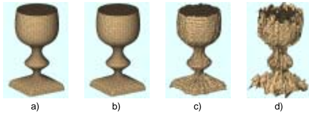
Figure 9: Compression of a B-spline surface with different quantizations. No additional point removal is performed ( \epsilon = 0 ). Some triangles degenerate due to quantization. a) 50% coefficients, 23 bit quantization, compression gain 1:1.33. b) 10 bit, 1:4. c) 7 bit, 1:5. d) 5 bit, 1:10. (Data source: Courtesy Advanced Visual System Inc. )
