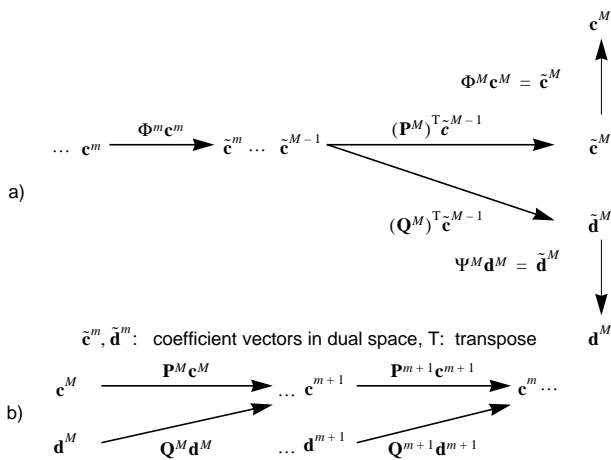
Figure 3: Linear time decomposition and reconstruction pyramids for cardinal B-spline wavelet transforms a) decomposition. b) reconstruction.
