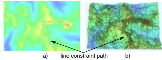
Figure 10: Illustration of constraints in a digital terrain data set. a) Interactive specification of the constraint path. b) Mesh after constraint insertion. (Data source: Courtesy Bundesamt für Landestopographie , Bern, Switzerland)
