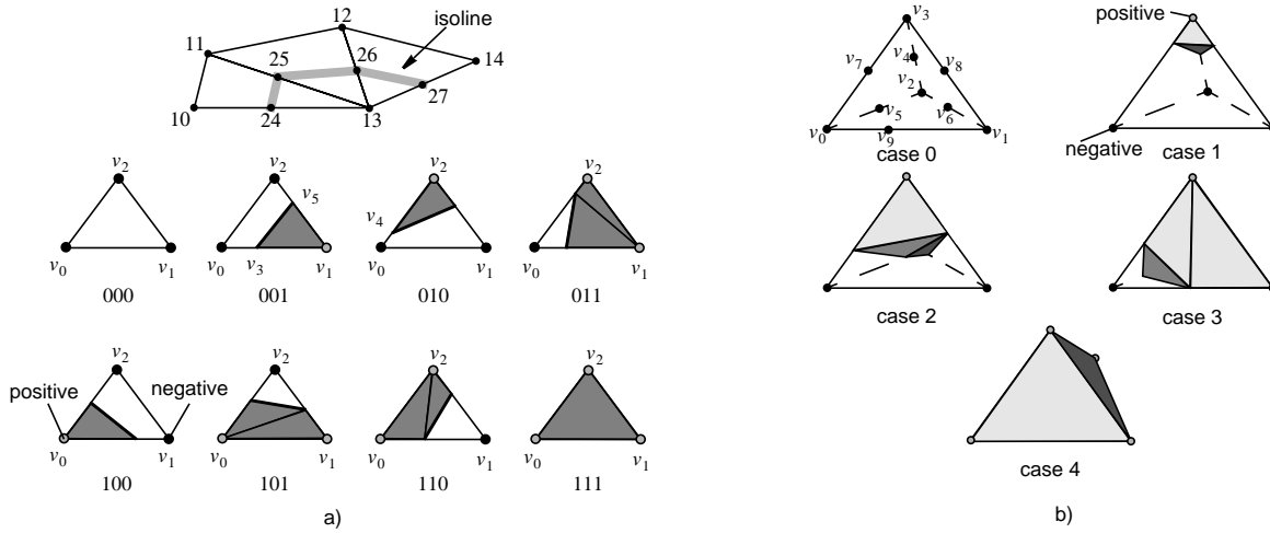
Figure 16: Polyline approximation of isolines: a) Isolines as computed by intersections with the triangle edges and look-up table to extract interior or exterior parts of the surface. b) Generation of isosurfaces and interior volumes using a marching tetrahedron algorithm: 5 basis cases arising upon triangulation. The connectivity table for generation of interior volumes is presented in Table 3.
