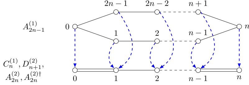
FIGURE 1. The diagram folding of type \widehat{\mathfrak{g}} = A_{2n-1}^{(1)} onto type \mathfrak{g} = C_n^{(1)}, D_{n+1}^{(2)}, A_{2n}^{(2)}, A_{2n}^{(2)\dagger} .
