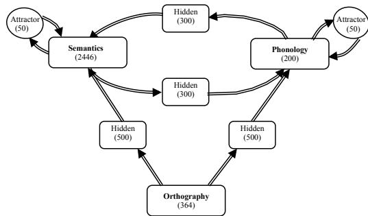
Figure 2. The architecture of the developmental model of reading.
