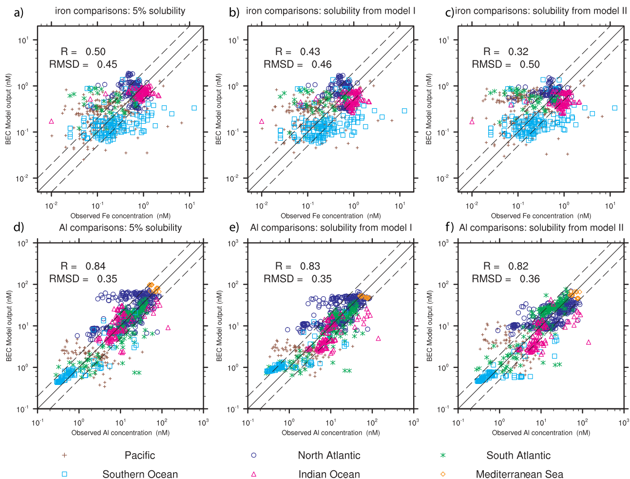
Figure 6. Dissolved Fe and Al concentrations predicted by the BEC models with different solubility fields compared to observations.
