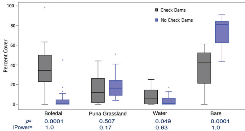
Figure 3. Percent cover of bofedal vegetation, Puna grassland, water, and bare substrate (including bedrock, sand and gravel, and cobbles) in gullies with check dams and gullies without check dams. The box-and-whisker plots show the median, 75th percentile, 25th percentile, and maximum–minimum values, with outliers symbolized with an x . Data are from four 25-m line transects established in each gully, and transects were established in five gullies with check dams and five gullies without check dams ( n = 5 \times 4 \times 2 ). The p -values are from a Brown–Forsythe one-way ANOVA, following a Levene’s F -test for equality of variances.
