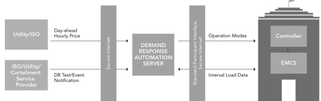
Fig. 1. Customer-side Transactions with Utilities and System Operators (Source: Lawrence Berkeley National Laboratory, DRRC Annual Report)
