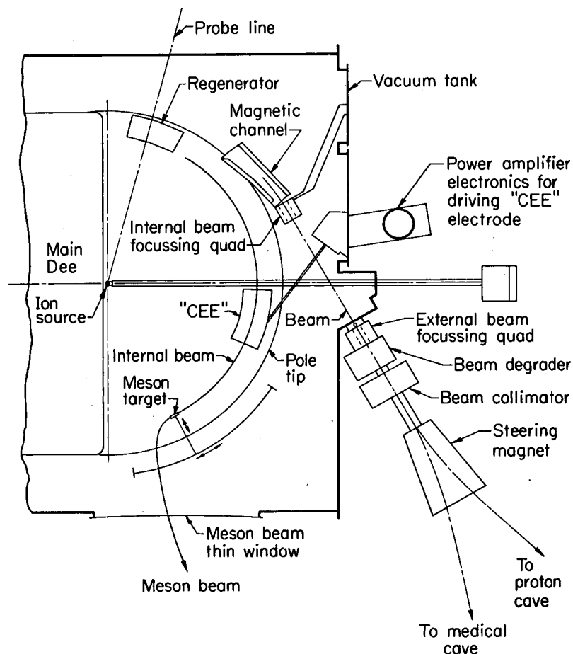
Fig. 2. Cyclotron Beam Component Arrangement
