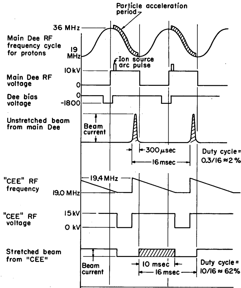
Fig. 1. Timing Sequence of Main Dee and "Cee"
