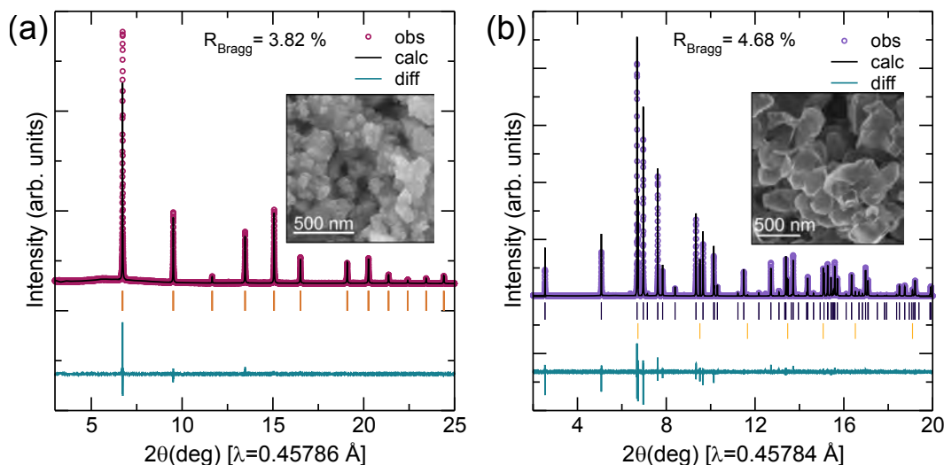
Fig. 2 Rietveld refinement of synchrotron XRD data of NbO 2 F (a) showed phase pure product while refinement of Nb 3 O 7 F (b) revealed a small impurity of less than 1% NbO 2 F, illustrated by the orange reflections. Both compounds have small particle sizes, as shown in SEM imaging (insets).
