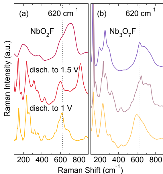
Fig. 6 (a): The Raman spectra of pristine \text{NbO}_2\text{F} as well as \text{NbO}_2\text{F} discharged to 1.5 V and 1.0 V, shows the disappearance of several modes followed by the introduction of new modes. (b) The Raman spectra of \text{Nb}_3\text{O}_7\text{F} , at various points of discharge, shows better maintenance of the modes seen in the pristine \text{Nb}_3\text{O}_7\text{F} .
