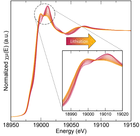
Figure S10: Nb K-edge X-ray absorption spectroscopy shows the characteristic down-shift of the K-edge associated with Nb reduction as \text{NbO}_2\text{F} is lithiated.
