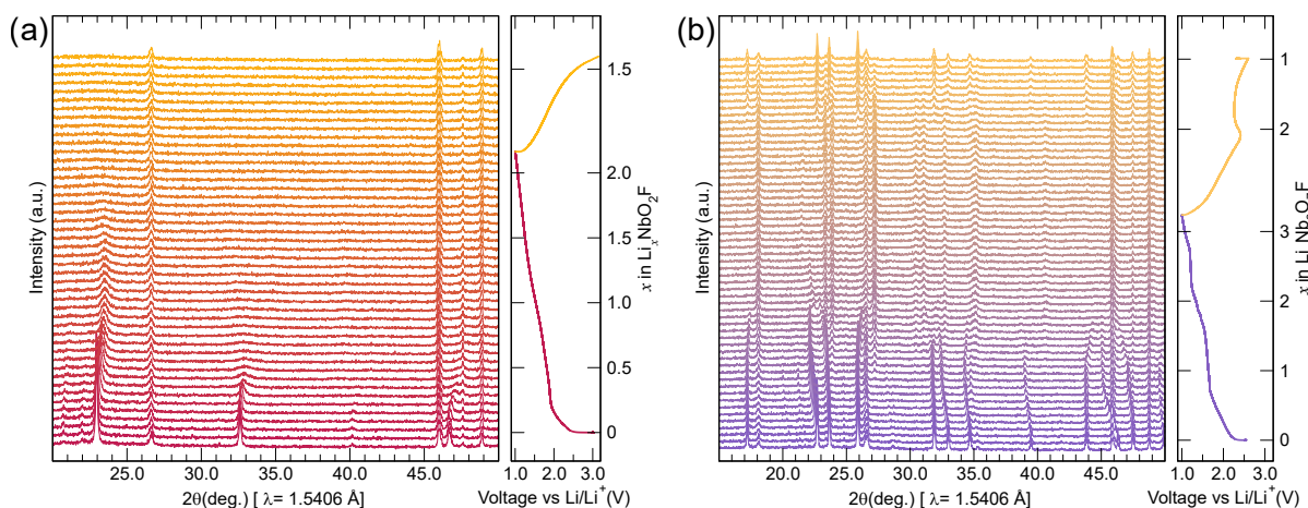
Fig. 4 Operando XRD measurements of \text{NbO}_2\text{F} (a) throughout a complete discharge/charge cycle reveals the loss of crystallinity induced by lithiation to \text{Li}_2\text{NbO}_2\text{F} . The loss of intensity on diffraction peaks is not recovered upon charging. In comparison, the structure of \text{Nb}_3\text{O}_7\text{F} (b) is seen to go through multiple changes during lithiation followed by a complete recovery upon charging, albeit with lowered crystallinity.
