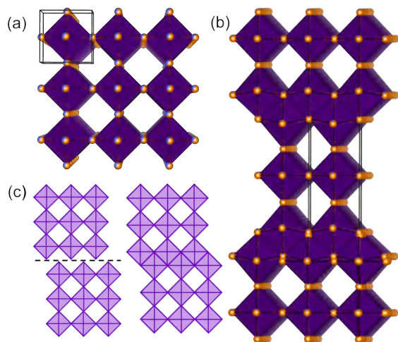
Fig. 1 (a): NbO 2 F exists in a perovskite structure with corner sharing octahedra. (b): Nb 3 O 7 F contains layers of edge sharing and corner sharing octahedra formed by the removal of an anionic plane of atoms from the perovskite structure. (c): Representative diagram of the shear relationship between NbO 2 F and Nb 3 O 7 F.
