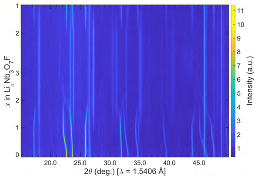
Figure S7: A heatmap of operando XRD for \text{Nb}_3\text{O}_7\text{F} demonstrates the differences in behavior during discharge and charge. During discharge, a solid solution type process is observed with steady peak shift throughout lithiation. During charging, growth of \text{Nb}_3\text{O}_7\text{F} is observed without the solid solution behavior seen on discharge.
