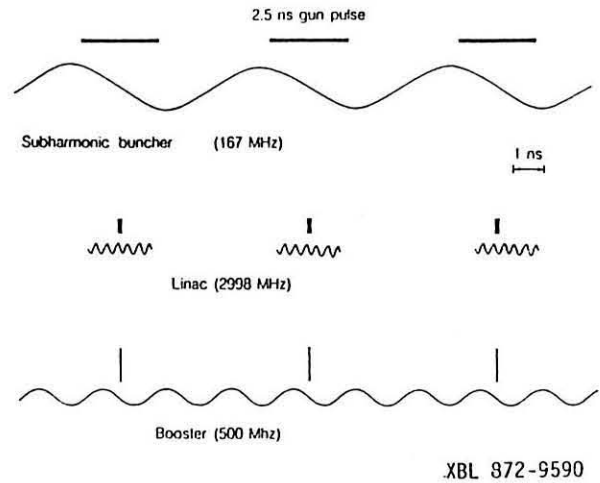
Fig. 2. Relation of beam bunches to rf in the subharmonic buncher, linac, and booster.
