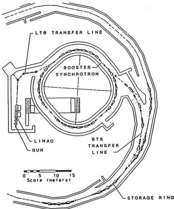
Fig. 1. Injection System Layout.
