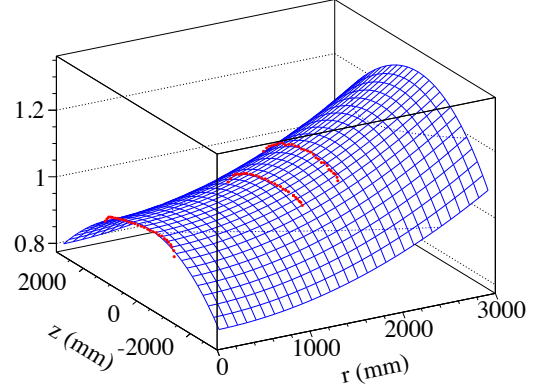
FIG. 7. Variation in light yield versus vertical ( z ) and radial ( r ) position of an interaction within EHI-AD1 for reconstruction A (blue surface). The functional form of the variation f_b(z, r) was motivated by simulation, and constrained using the relative light yield of ^{60}\text{Co} calibration data from ACU A ( r=0 mm), ACU B ( r=1350 mm) and ACU C ( r=1772.5 mm) (red points). While the modeled correction was between -6% to 17% over the volume of a detector, only slight differences ( <3.2\% ) were observed between the eight detectors.
