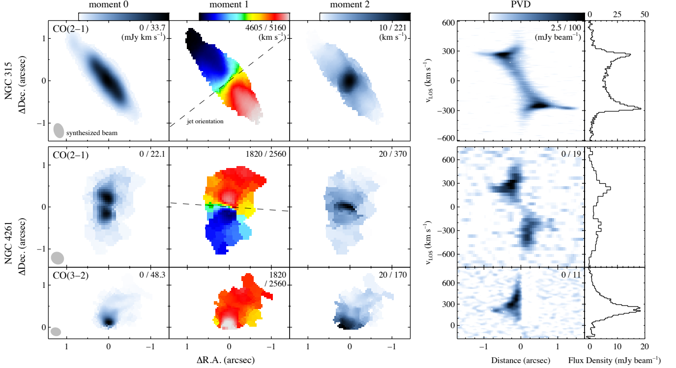
Figure 6. Moment maps constructed from NGC 315 CO(2–1) ( top panels ) and NGC 4261 CO(2–1) and CO(3–2) ( middle/bottom panels ) ALMA data cubes. The moment maps reveal regular, albeit slightly warped, disk rotation. In the outer disk regions, spectra were binned together to achieve higher S/N. The moment values are linearly mapped to colors, shown by the color bar to the top of the maps, and the ranges in each panel indicate the minimum and maximum values of each color bar. The orientation of the radio jets ( dashed lines ) are roughly perpendicular to the lines of nodes. Major-axis position-velocity diagrams (PVDs; right panels ) are displayed with their v_{\text{LOS}} relative to v_{\text{sys}} from Table 3, with color bar ranges in each panel. Velocity profiles ( far right panels ) for each cube were constructed by integrating flux densities within mask regions that follow the emission observed in each channel.
