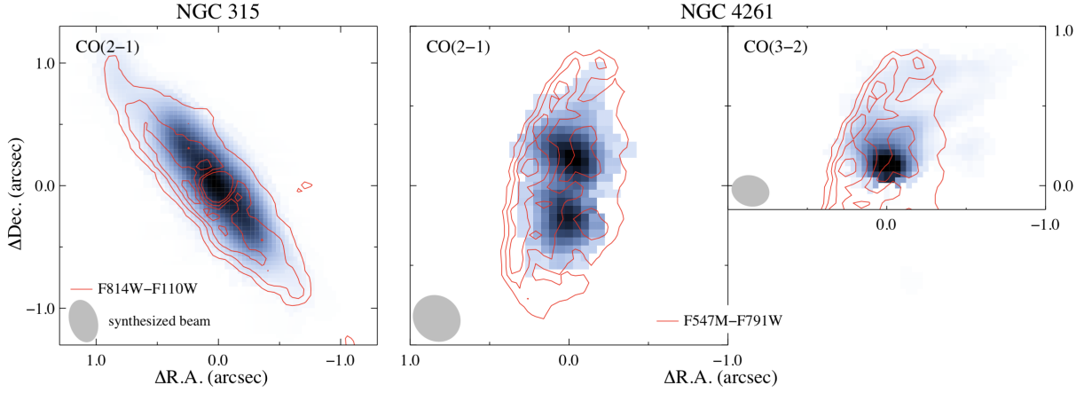
Figure 5. CO(2–1) and CO(3–2) zeroth moment maps measured from the NGC 315 and NGC 4261 ALMA data sets. The frequency range of the archival NGC 4261 CO(3–2) observations excludes most of the emission on the approaching (south) side of the disk. Contours show the respective HST I-J and V-I colors. The CO emission in each galaxy is concentrated within the region enclosed by the maximum HST color contours.
