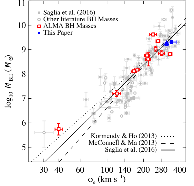
Figure 11. Comparison between dynamically measured BH masses and host galaxy \sigma_e (filled gray circles: Saglia et al. 2016), along with other literature values (open gray circles: den Brok et al. 2015; Greene et al. 2016; Thomas et al. 2016; Walsh et al. 2016, 2017; Erwin et al. 2018; Krajnović et al. 2018; Mehrgan et al. 2019; Liepold et al. 2020) and those measured using ALMA observations (colored squares: Barth et al. 2016a; Onishi et al. 2017; Davis et al. 2017, 2018; North et al. 2019; Smith et al. 2019; Nagai et al. 2019; Boizelle et al. 2019; Ruffa et al. 2019b; Davis et al. 2020; Nguyen et al. 2020). When not listed in the papers, we adopted \sigma_e values and/or uncertainties when available from other sources (Barth et al. 2002; Filippenko & Ho 2003; Brough et al. 2007; Cappellari et al. 2013; Kormendy & Ho 2013; Ma et al. 2014; Saglia et al. 2016; van den Bosch 2016; Veale et al. 2017). The NGC 315 and NGC 4261 BH masses presented here are consistent with M_{\text{BH}} - \sigma_e relations from Kormendy & Ho (2013), McConnell & Ma (2013), and Saglia et al. (2016).
