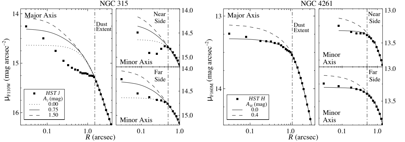
Figure 4. Comparison between the observed NGC 315 J and NGC 4261 H -band surface brightness profiles and those derived from extinction-corrected MGE models. For NGC 315, we show both the dust-masked ( A_J = 0 mag) model and MGEs constructed after correcting central surface brightness values for A_J = 0.75 and 1.50 mag of extinction of the light behind the disk. For NGC 4261, we show the dust-masked ( A_H = 0 mag) model along with an MGE solution corrected for a central extinction of A_H = 0.4 mag. The minor axis plots ( right-hand panels ) show NGC 315 and NGC 4261 surface brightness profiles taken along the near (southeast and east of the nuclei, respectively) and far sides of the dust disks. We note that the central J and H -band excesses are fit as point sources with no extinction correction and are not included in the MGE models.
