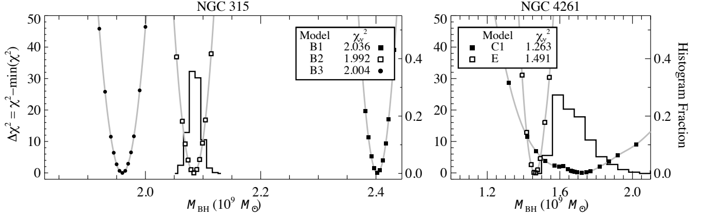
Figure 9. Results from \chi^2 minimization as a function of BH mass for the NGC 315 CO(2–1) and NGC 4261 CO(2–1) and CO(3–2) dynamical models. Gray lines are spline interpolations to the \Delta\chi^2 = \chi^2 - \min(\chi^2) values. The histograms show the distributions of BH masses determined from Monte Carlo resampling of the B2 and C1 best-fit model cubes.
