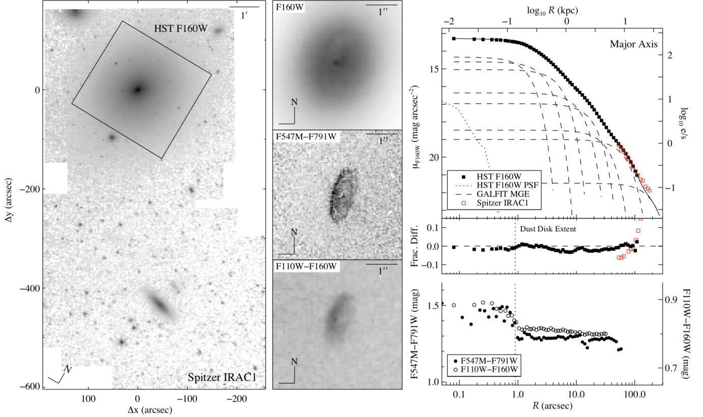
Figure 2. Optical to mid-IR imaging of NGC 4261. The HST WFC3 F160W image is overlaid on a Spitzer IRAC1 mosaic ( left panel ), shown using a logarithmic intensity scale. The F547M–F791W and F110W–F160W color maps (shown in central 4''.1 \times 4''.1 cut-out regions; middle panels ) reveal a round circumnuclear dust disk that is slightly miscentered relative to the stellar bulge. The luminous mass model for this galaxy was constructed by parameterizing the H -band surface brightness using a GALFIT MGE and a central point source component ( top right panel ). These HST measurements were augmented with larger-scale IRAC1 data. The ( A_H = 0 mag) MGE solution shown here and in Table 1 was derived after masking the reddest IR colors in the H -band cutout, which are expected to trace the most dust-obscured regions.
