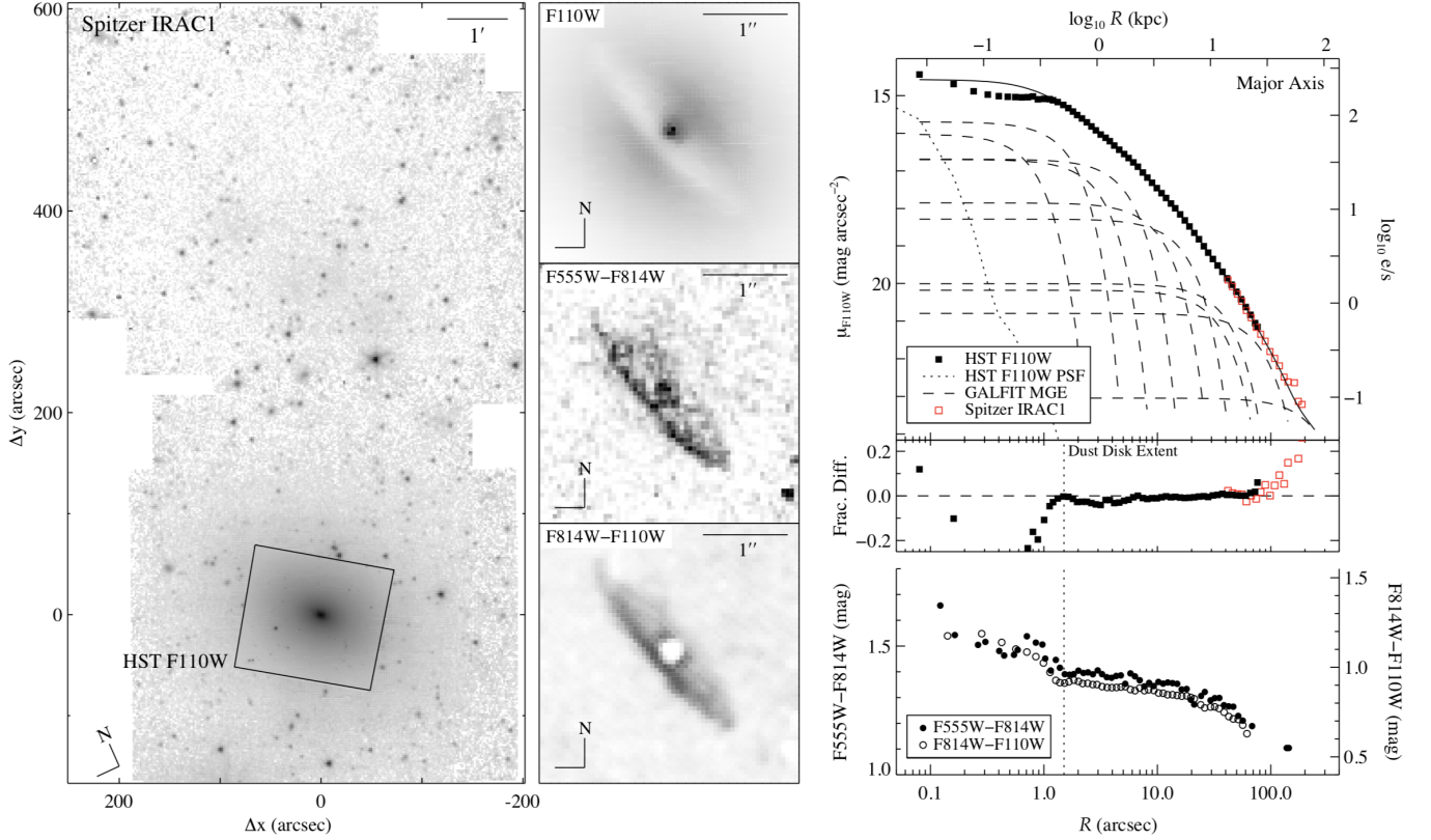
Figure 1. Optical to mid-IR imaging of NGC 315. The HST WFC3 F110W image is overlaid on a Spitzer IRAC1 mosaic ( left panel ), shown using a logarithmic intensity scale. F555W–F814W and F814W–F110W color maps (shown in central 4''.1 \times 4''.1 cut-out regions; middle panels ) trace a morphologically regular and highly inclined dust disk. Luminous mass models for this galaxy were constructed by parameterizing the J -band stellar surface brightness using a GALFIT MGE ( top right panel ) accompanied by a nuclear point-source component. Here, we augmented the HST measurements with larger-scale IRAC1 data. The ( A_J = 0 mag) MGE solution shown here and in Table 1 was derived after masking the most dust-obscured regions seen in the J -band cut-out.
