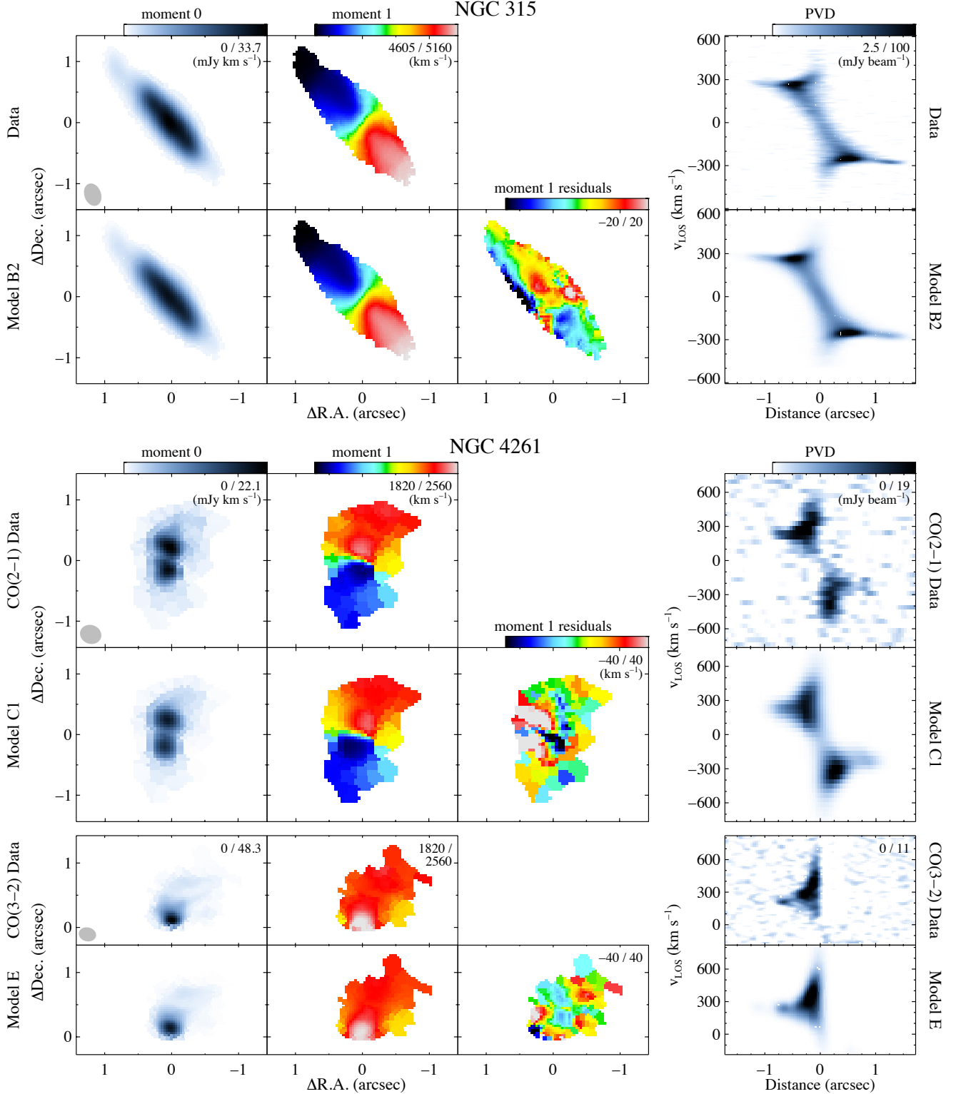
Figure 7. Comparison between the luminosity-weighted NGC 315 CO(2-1) ( top panels ) and NGC 4261 CO(2-1) and CO(3-2) ( middle/bottom panels ) zeroth and first moment maps and PVDs with those derived from best-fitting models B2, C1, and E. With the noticeable exception of model C1 for NGC 4261, the first moment residual maps show generally small deviations ( \lesssim 10 km s -1 , or 4%) between data and the best-fit models, with the largest discrepancies near the disk center. Likewise, the model PVDs generally agree with the data. However, model B2 for NGC 315 underrepresents the CO(2-1) emission that has |v_{\text{LOS}} - v_{\text{sys}}| \gtrsim 350 km s -1 , and model C1 for NGC 4261 cannot reproduce the sharp velocity upturn seen in the approaching side of the disk.
