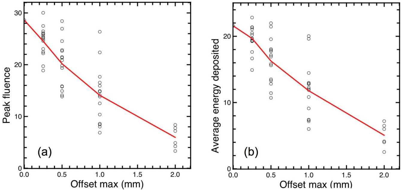
FIG. 12: Energy fluence ( \text{J}/\text{cm}^2 ) at focal plane versus amplitude of random offsets of solenoid ends (flat distribution with maximum shown on abscissa), from ensembles of 3-D Warp simulations (without steering dipoles): (a) peak deposition, time integrated; (b) average over circle of 0.1 mm diameter surrounding brightest spot, gated in time to include only central nanosecond around peak.
