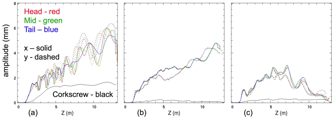
FIG. 13: (color online) ASP studies of steering (in an extended version of NDCX-II), showing RMS values of x (solid lines) and y (dashed lines) centroid coordinates vs. z for head, middle, and tail particles, and the corkscrew amplitude; the results are averages over 20 simulations with differing random offsets of solenoid ends up to 1 mm. Dipole magnets and sensors were placed in every fourth cell, and the penalty function was evaluated at the next sensor downstream from the dipole being varied. (a) without steering; (b) with steering optimization that penalizes corkscrew amplitude; (c) with steering optimization that penalizes corkscrew amplitude and beam offset, and constrains dipole fields to less than 100 G.
