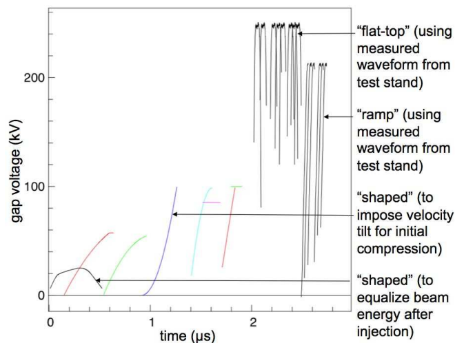
FIG. 4: (color online) Waveforms for acceleration from ASP.
