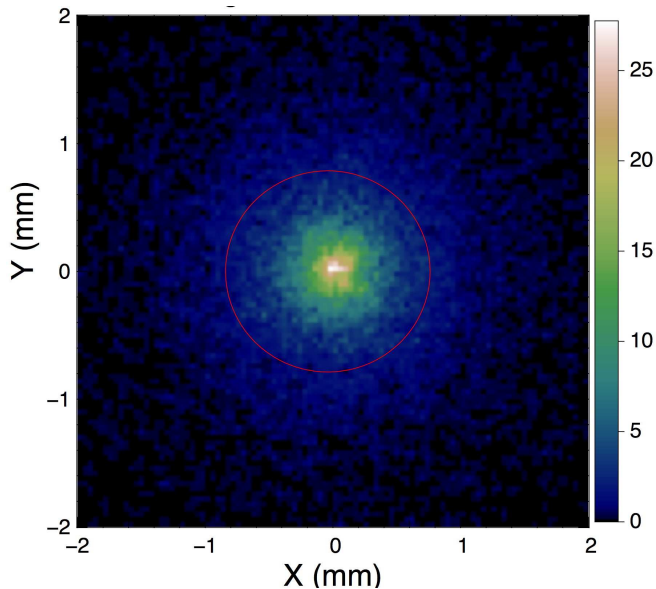
FIG. 8: (color online) Energy deposition into target plane at z = 13.15 m from Warp in (r, z) geometry; colorbar denotes \text{J}/\text{cm}^2 ; semi-axes of ellipse equal RMS extents in x and y .
