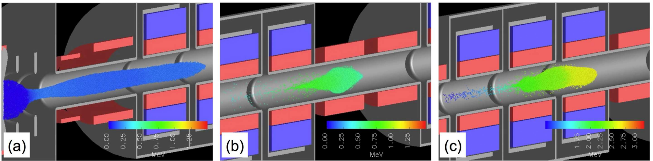
FIG. 11: (color online) Images from a video depicting the beam in a 3-D Warp simulation of NDCX-II; as in Fig. 10, but the system is assumed to be misaligned, with random transverse offsets of solenoid ends up to 2 mm (enhanced online).
