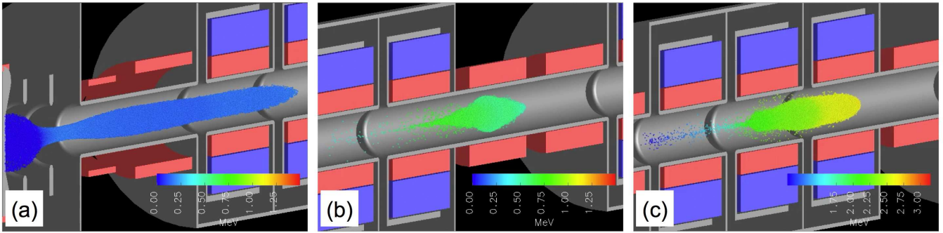
FIG. 10: (color online) Images from a video depicting the beam in a 3-D Warp simulation of NDCX-II; colorbars denote ion kinetic energy. The induction cores (blue color) are not shown to true scale - their radial extent is compressed by a factor of two, so as to allow the orientation of the induction cells to be seen. The red shapes denote the volumes occupied by the solenoids and their flux return channels. The system is assumed perfectly aligned, and the beam is shown (a) emerging from the injector; (b) after gap 8; and (c) passing through gap 16 (enhanced online).
