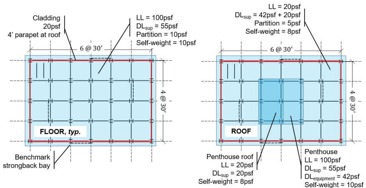
Figure 5.3. Gravity loading.
