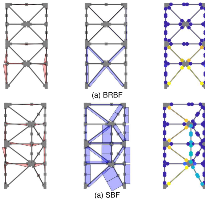
Figure 6.32. SBF and BRBF comparison – Response diagram at time of peak story shear for gm44.
