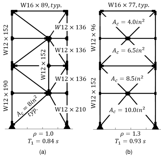
Figure 5.14. (a) benchmark embedded SBF, (b) reference BRBF.
