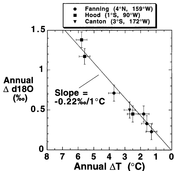
FIG. 2. Correlation between annual range in historical sea surface temperature (SST) records ( \Delta T^{\circ}\text{C} ) and annual range in \delta^{18}\text{O} values ( \Delta \delta^{18}\text{O} ) in coral bands from the Galapagos Islands, Fanning Island, and Canton Island. The line shown represents a slope of 0.22\text{‰} per 1\text{°C} decrease in SST predicted by the temperature-dependent aragonite-water fractionation factor. This slope is the same as that defined for the equilibrium precipitation of calcite (66). (Data are from ref. 69.)
