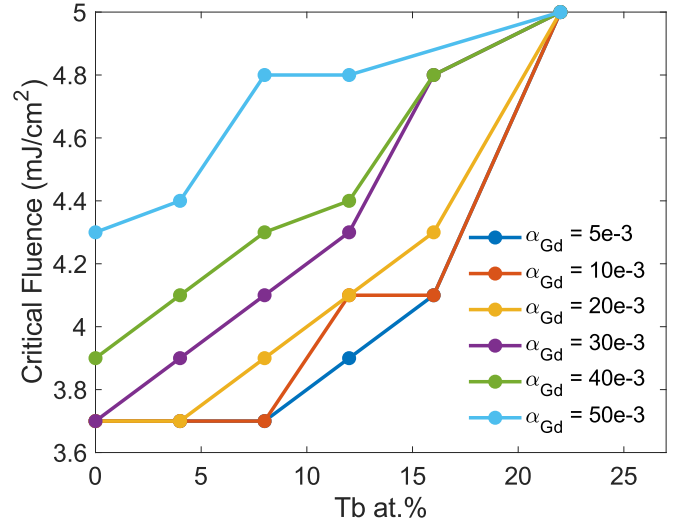
FIG. 3. Simulated critical fluence of a -Gd 22-x Tb x Co 78 films as a function of Tb at. % x for different damping values of Gd, \alpha_{Gd} . The Tb and Co damping parameters are constant (0.05). The critical fluence increases as \alpha_{Gd} increases, indicating that lowering \alpha_{Gd} reduces the threshold switching condition of a -Gd-Tb-Co alloys below the laser ablation limit.
