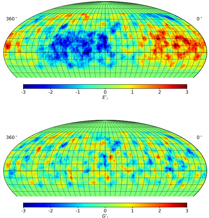
Figure 3. Simulated event excess in f_1 for an injected signal which mimics the cosmic-ray anisotropy, smoothed with a 5^\circ tophat. Top : Event excess after subtracting the estimated background from the simulated data. Bottom : Large-scale structure dominated by cosmic rays is removed after the method described in Section 3.2 is applied.
