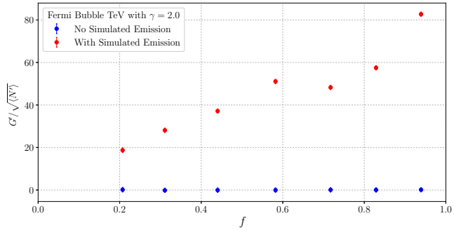
Figure 5. Simulated event excess over the square-root of the isotropic background inside the Northern Bubble region without and with strong Fermi Bubble-like emission after applying the procedure. See method described in Section 3.2.
