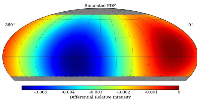
Figure 2. Dipole distribution used for the skymap simulation.
