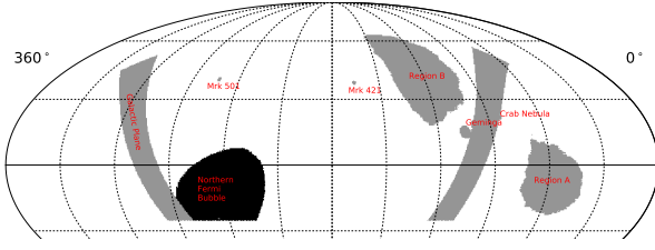
Figure 1. Skymap in equatorial coordinates showing the region of interest masking as used for the analysis. The masked ROI include the Galactic Plane, Geminga, the Crab Nebula, Mrk 421, Mrk 501, the small-scale anisotropies region A and B, and the Northern Fermi Bubble.
