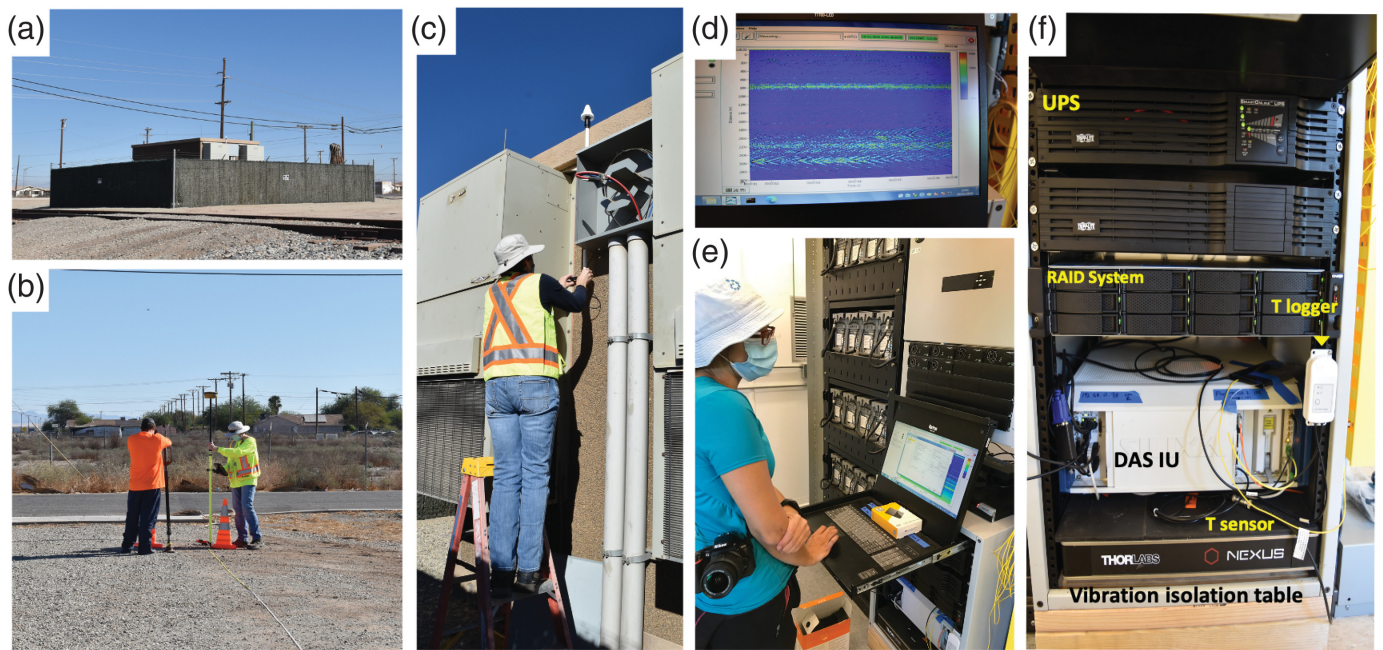
Figure 2. Field installation and system montage. (a,b) the Calipatria, California, intermediate light amplification (ILA) hut and a tap test location, respectively; (c) installation of the Global Positioning System antenna and external environmental monitoring sensor; (d–f) the first recorded data, interrogator unit (IU) configuration process, and IU monitoring system stack, respectively. UPS, uninterruptible power supply.
