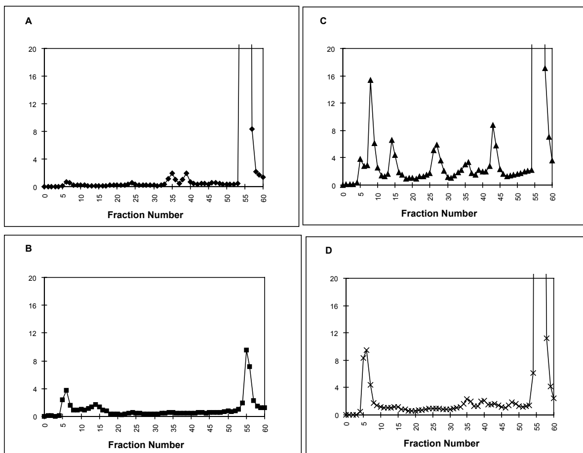
Figure 3: HPLC profile of organic extracts of (A) BaP medium before addition to transwell, (B) basolateral medium, (C) cell layer, and (D) apical medium 1 hour after addition of 0.2 \mu\text{M} ^3\text{H} -BaP to apical chamber. Peaks were identified by comparison to the elution of known BaP metabolite standards. Various tetrol and triol isomers are eluted in the first 18 fractions, followed by diols, then monol and finally BaP.
