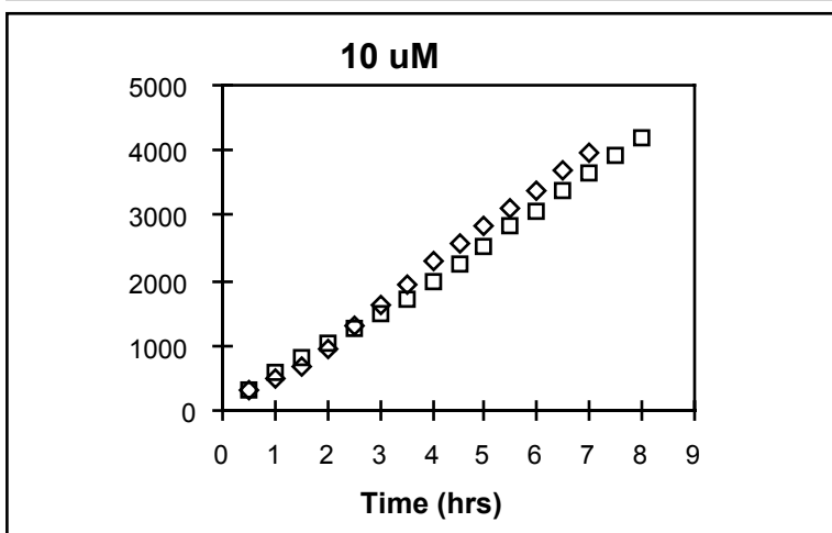
Figure 1: ^3\text{H} -BaP permeation of Caco-2 cell layers after BaP addition to apical chamber (top panel - 0.2 \mu\text{M} BaP, middle panel - 1 \mu\text{M} BaP, bottom panel - 10 \mu\text{M} BaP). Values from two independent experiments, each the mean of two transwells, are presented. In the first ( \diamond ) medium was collected and replaced through the sample port every 30 min
