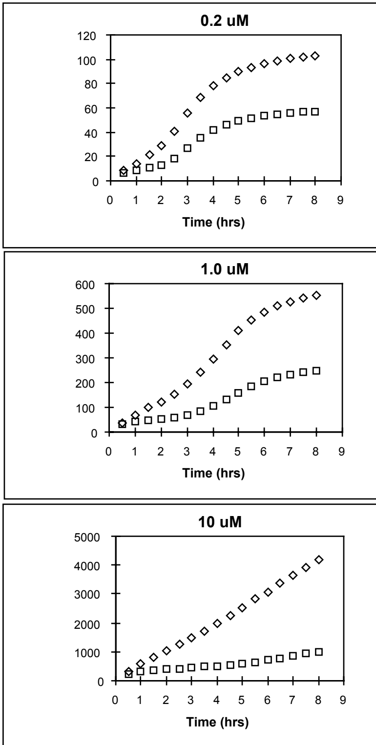
Figure 2: Water soluble BaP metabolites appearing in the basolateral chamber after addition of different concentrations of BaP to apical chamber (top panel - 0.2 \mu\text{M} BaP, middle panel - 1 \mu\text{M} BaP, bottom panel - 10 \mu\text{M} BaP). Total ^3\text{H} -activity recovered from
