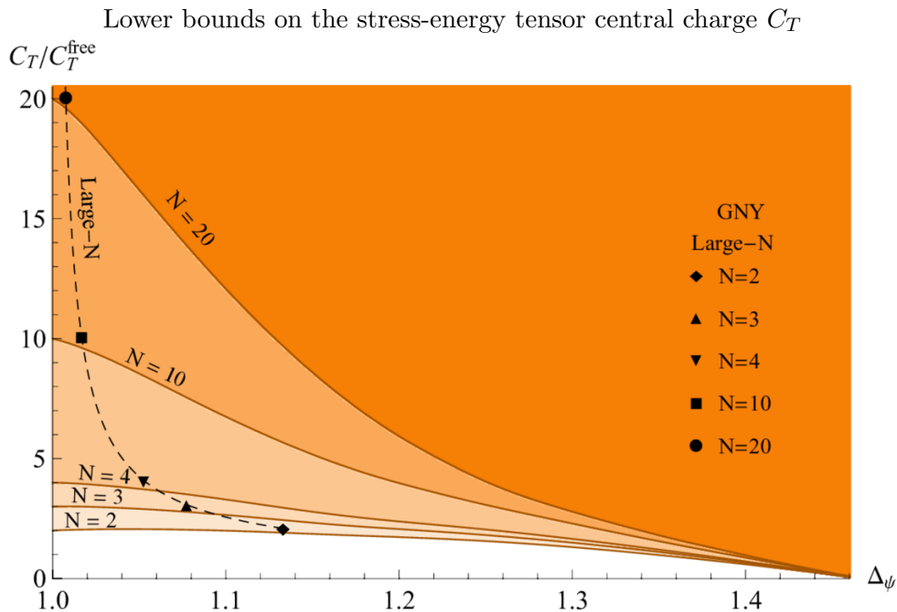
Figure 7. Lower bounds on the stress energy tensor central charge C_T as a function of the scaling dimension \Delta_\psi of the fermion transforming in the O(N) fundamental representation. We normalize the central charges C_T such that as \Delta_\psi \rightarrow 1 , we set the value of C_T to be equal to the number of fermions in the theory. The black markers are large- N estimates for GNY models obtained up to O(1/N^2) corrections [45].
