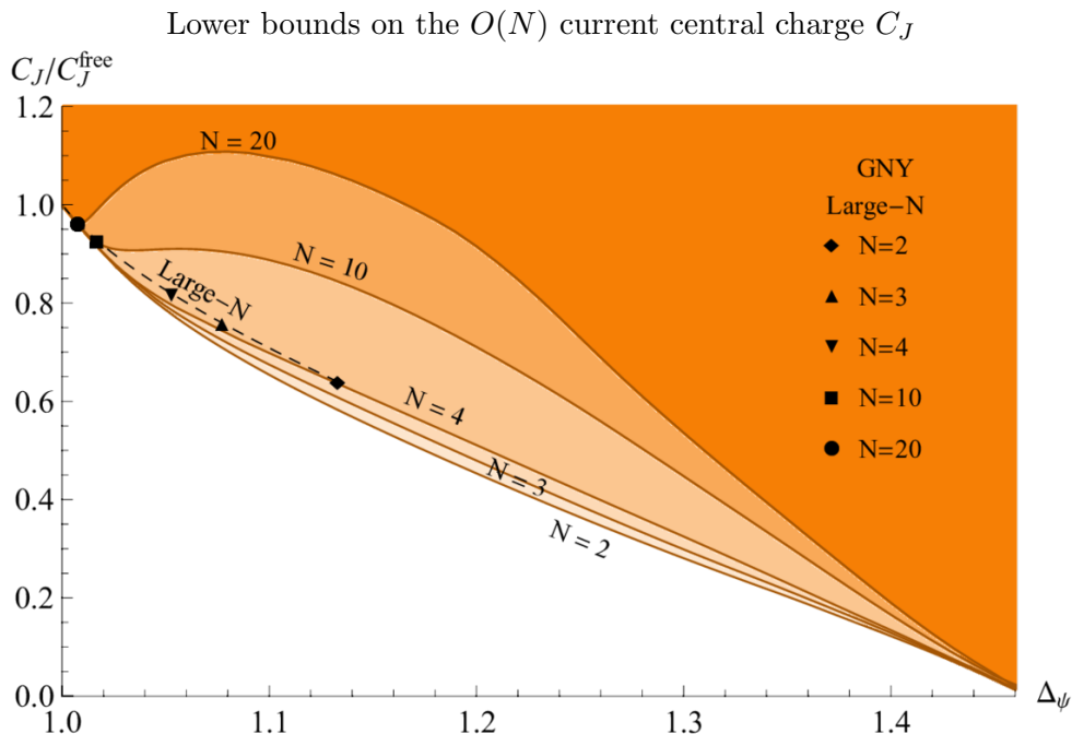
Figure 6. Lower bounds on the O(N) conserved current central charges C_J as a function of the scaling dimension \Delta_\psi . We normalize the central charges C_J such that as \Delta_\psi \rightarrow 1 , we set the value of C_J = 1 . For N = 10, 20 the bound has a local minimum that lies close to the large- N values of (\Delta_\psi, C_J) in GNY models obtained up to O(1/N^2) corrections (black markers) [45]. This is reminiscent of the central charge bound in the scalar bootstrap which had a local minimum corresponding to 3D Ising model. The bounds for smaller values of N have no similar features.
