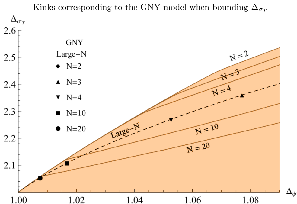
Figure 1. Upper bounds on the scaling dimension of the lowest-lying parity-odd O(N) symmetric-traceless tensor, \Delta_{\sigma_T} , for a unitary CFT containing fermions with scaling dimension \Delta_\psi . We focus on the cases N = 2, 3, 4, 10 and 20 . The black symbols show the estimated values of the scaling dimensions \Delta_\psi and \Delta_{\sigma_T} obtained from the large- N expansion up to O(1/N^4) corrections [28]. For N = 10, 20 we note strong agreement. This figure is a zoomed in version of figure 5.
