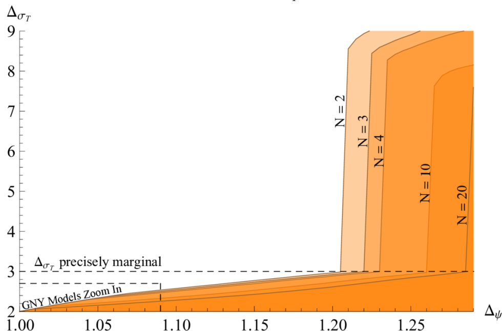
Figure 5. Upper bounds on the scaling dimension of the lowest-lying parity-odd O(N) symmetric-traceless tensor, \Delta_{\sigma_T} , for a unitary CFT containing fermions with scaling dimension \Delta_\psi . Once again, we focus on the cases N = 2, 3, 4, 10 and 20 . As \Delta_\psi \rightarrow 1 , the bound approaches the free theory value of \Delta_{\sigma_T} = 3 . There are two sets of kinks. The first set of kinks correspond to the GNY-models and are located in the square on the lower left. We zoom onto this lower left square in figure 1 and discuss the meaning of the kinks in more detail in section 4.
