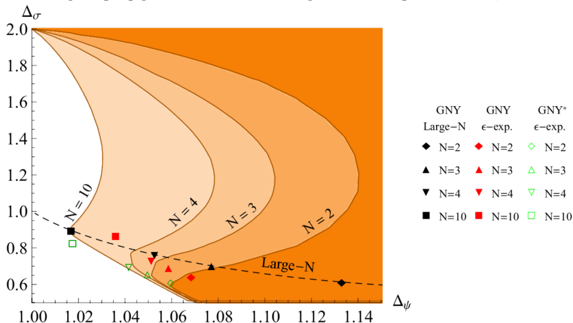
Figure 2. Bound on the scaling dimension of the lowest-lying parity-odd O(N) singlet, \Delta_\sigma , for a unitary CFT containing fermions with scaling dimension \Delta_\psi , when imposing a gap above this operator up to \Delta_{\sigma'} > 3 . Once again, we focus on the cases N = 2, 3, 4 , and 10 . We notice that when imposing such a gap, we observe features that are close to the values of \Delta_\psi found for the GNY kinks in figure 1. Estimates from the large- N expansion (black markers) for the scaling dimension of \Delta_\sigma also agree well with the position of the kink for N = 10 , but is inaccurate at smaller values of N . The red markers are the three-loop \epsilon -expansion results for the dimensions of the GNY models after performing a \text{Pade}_{[2,1]} approximation (see eqs. (11)–(13) and table II in [33]). They are reasonably close to the upper kinks in the bounds for small N . The lower kinks appear close to the three-loop \epsilon -expansion estimates for the GNY* models (green hollow markers), obtained after performing a \text{Pade}_{[1,2]} approximation, following the methods in [28] and [33]. While these second kinks are close to the \epsilon -expansion estimates for small N , for N = 10 the second kink does not exist at all.
