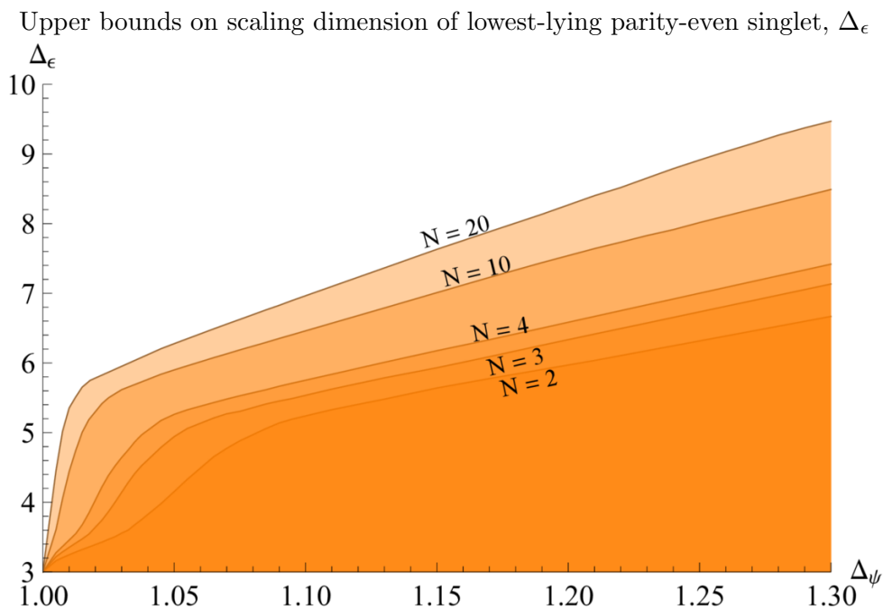
Figure 4. Upper bounds on the scaling dimension of the lowest-lying parity-even O(N) singlet, \Delta_\epsilon , for a unitary CFT containing fermions with scaling dimension \Delta_\psi . Once again, we focus on the cases N = 2, 3, 4, 10 and 20 . As \Delta_\psi \rightarrow 1 , the bound approaches the value of \Delta_\epsilon = 3 .
