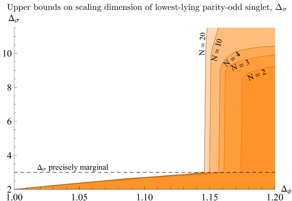
Figure 3. Upper bounds on the scaling dimension of the lowest-lying parity-odd O(N) singlet, \Delta_\sigma , for a unitary CFT containing fermions with dimension \Delta_\psi . Above, we focus on the cases N = 2, 3, 4, 10 and 20 . As \Delta_\psi \rightarrow 1 , the bound approaches the free theory value of \Delta_\sigma = 2 . Reminiscent of the jump noticed in our previous work [13] when bounding the scaling dimension of the lowest-lying parity-odd operator in a theory with one fermion, we observe a different jump for each value of N that we study. Once again, all jumps occur once the bound intersects the horizontal line on which \sigma is precisely marginal, \Delta_\sigma = 3 .
