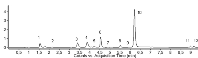
Figure 2. Total ion chromatogram of a mixture of the studied compounds. The numbers assigned to each peak correspond to each of the studied compounds.
