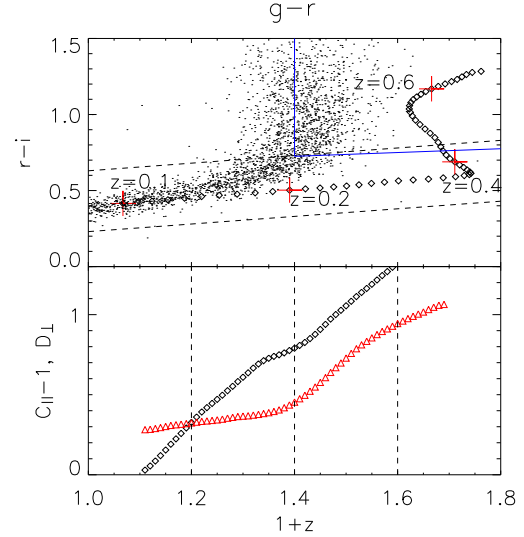
Figure 2. The top panel shows simulated g-r and r-i colours of an early-type galaxy as a function of redshift. The spectrum used to generate the track is the same as in Fig. 1, but evolved in redshift. Also shown are the colour cuts for Cut I (dashed, black) and Cut II galaxies (solid, blue). The points show the stellar locus as determined by a sample of stars with r -band magnitudes less than 19.5. The lower panel shows the colours c_{||} (diamonds, black) and d_{\perp} (triangles, red), as a function of redshift. Also shown are fiducial redshift boundaries for Cut I (0.2 – 0.4) and Cut II (0.4 – 0.6). Note that the range in g-r is identical to the range in 1+z .
