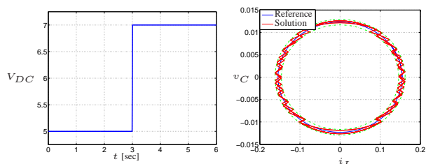
(b) V_{DC} signal. (c) Corresponding trajectory of proposed controller.
