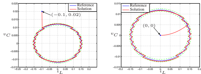
(a) Solution to initial condition outside S_o . (b) Solution to initial condition inside S_i .
