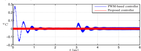
(a) v_C output of the single-phase inverter with PWM-based and proposed hybrid controllers for V_{DC} with a step at 3s.
