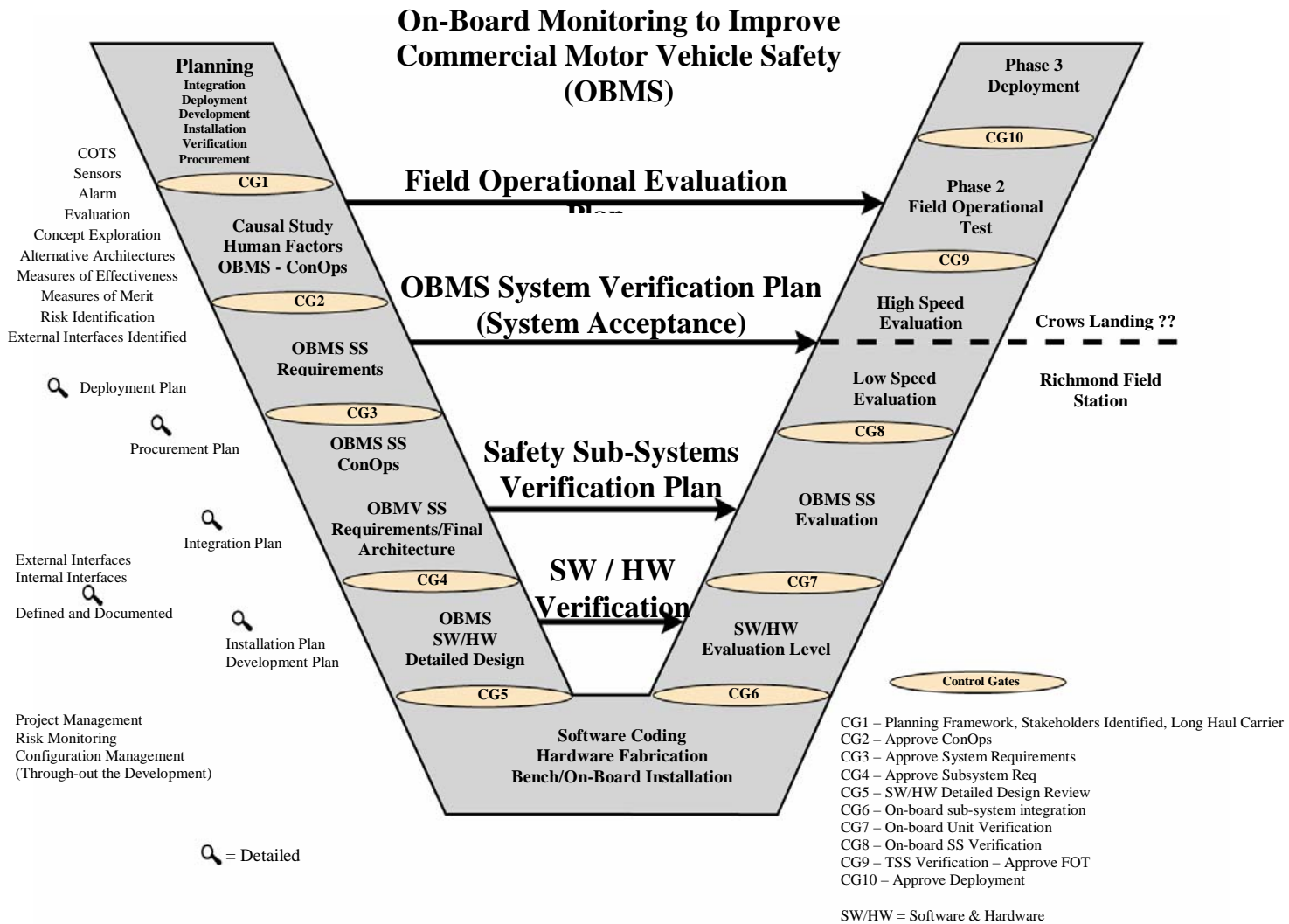
Figure 7-1. Project Vee Diagram
