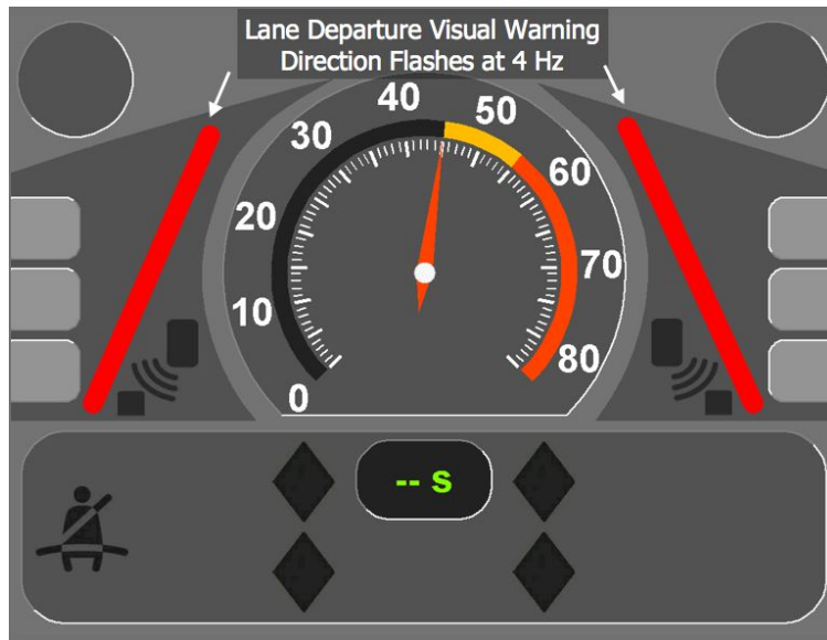
Figure 5-4. OBMS Prototype Lane Departure Warning Visual Feedback Design
