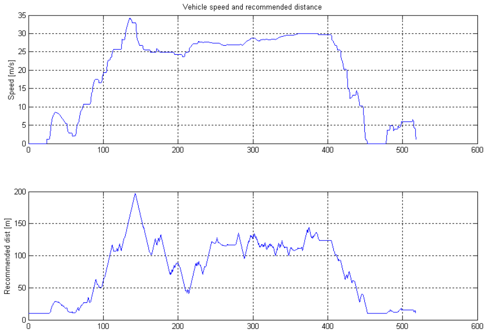
Figure 4-1. Truck Speed vs. Recommended Distance
