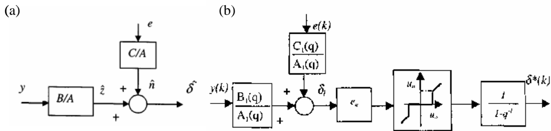
Figure 4-5. Driver Model Using ARMAX Structure
