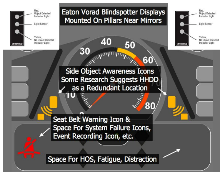
Figure 5-5. OBMS Prototype Visual Feedback Design for Seat Belt and Side Obstacles
