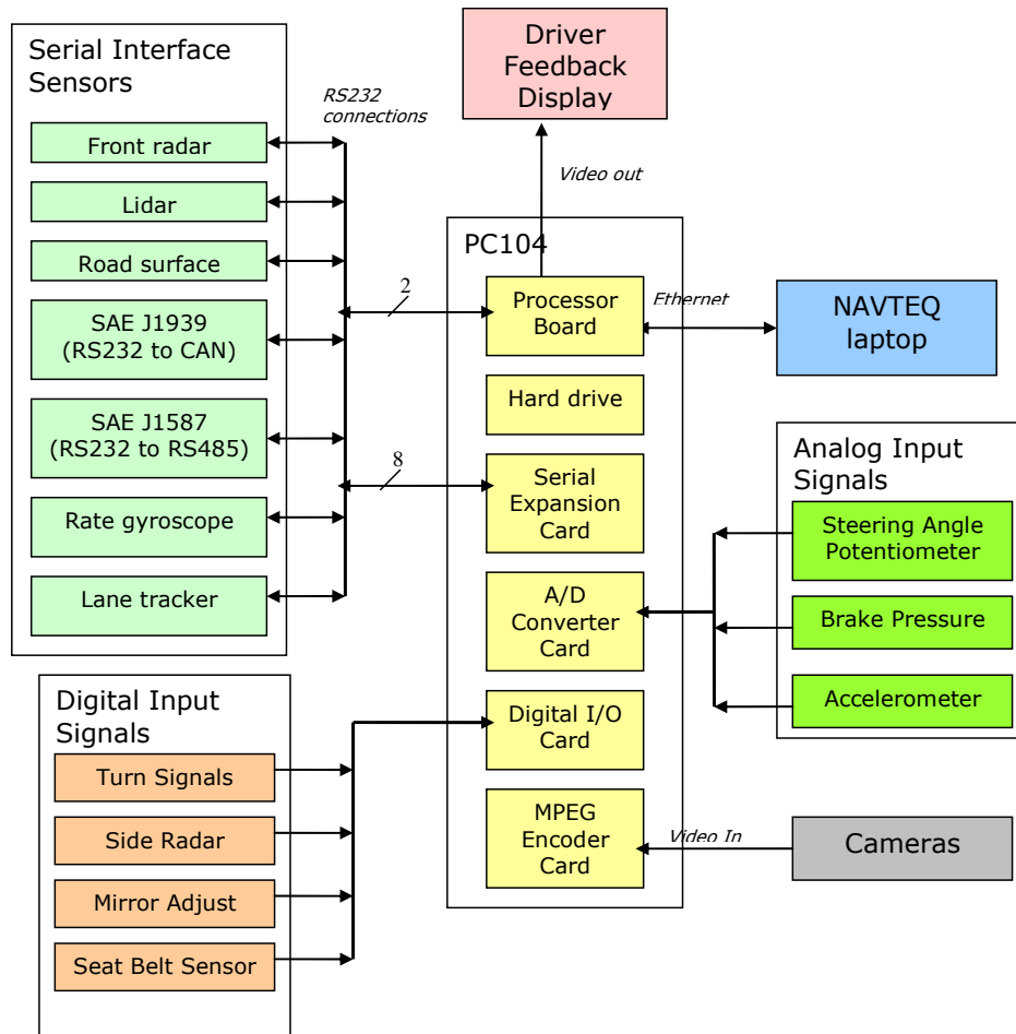
Figure 7-1. Block Diagram of OBMS Prototype PC104 and Sensor Interfaces
