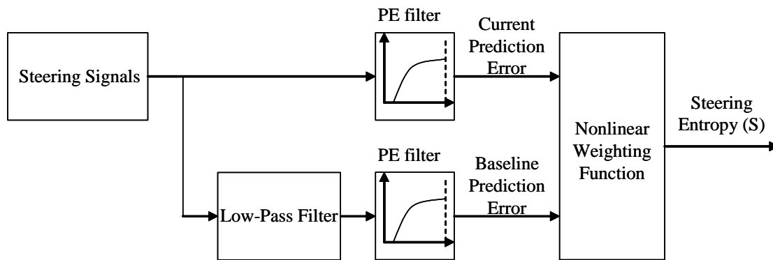
Figure 4-10. Block Diagram of Implemented Inattention Detection Algorithm
