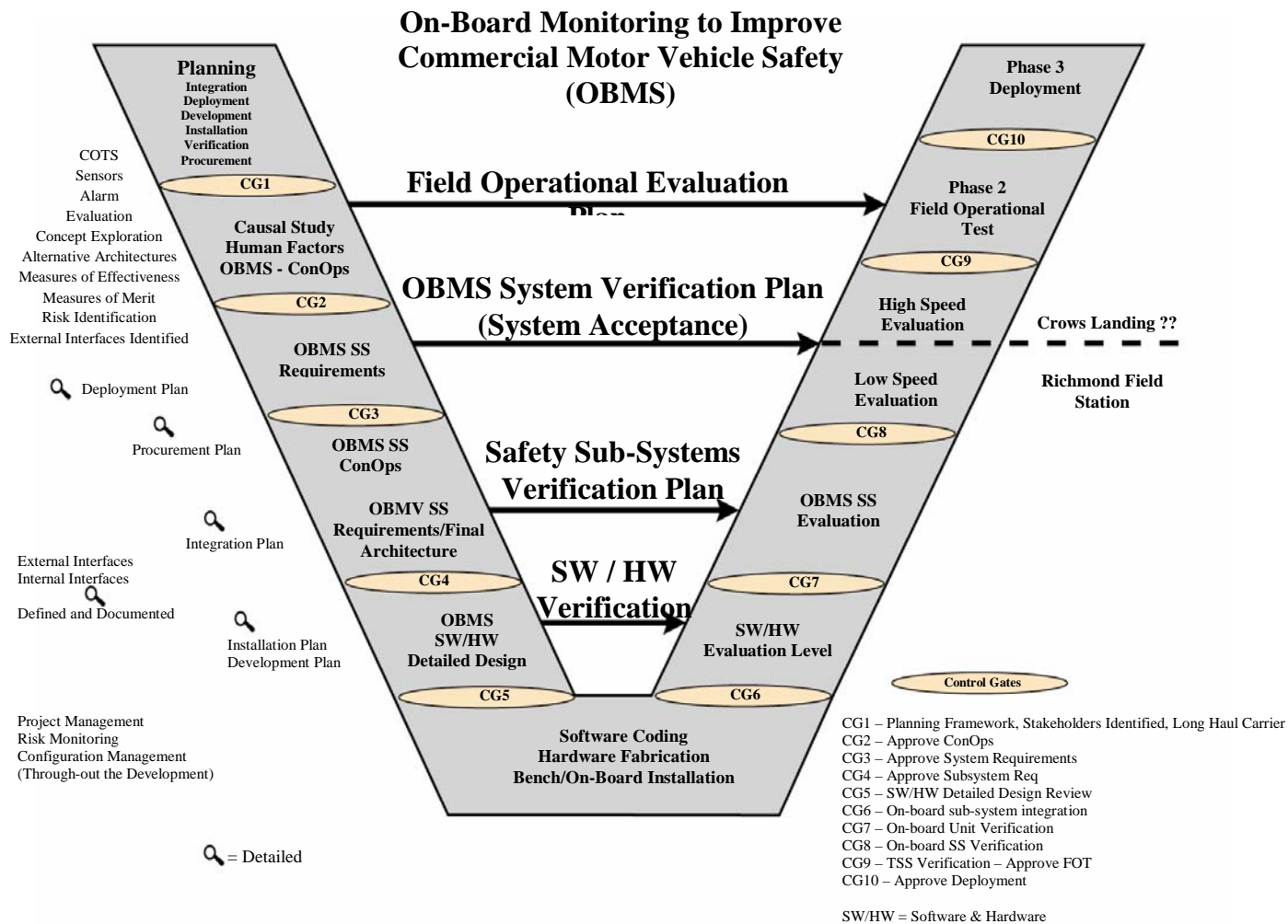
Figure 1-1. Project Vee Diagram
