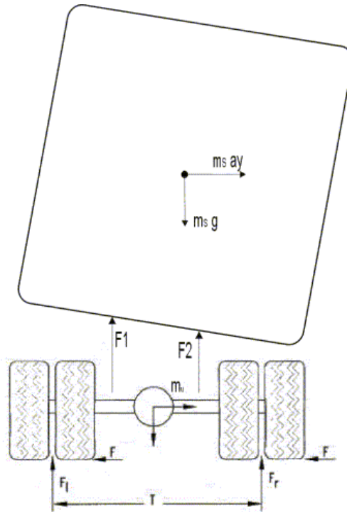
Figure 4-2. Vehicle Sprung Mass Model
