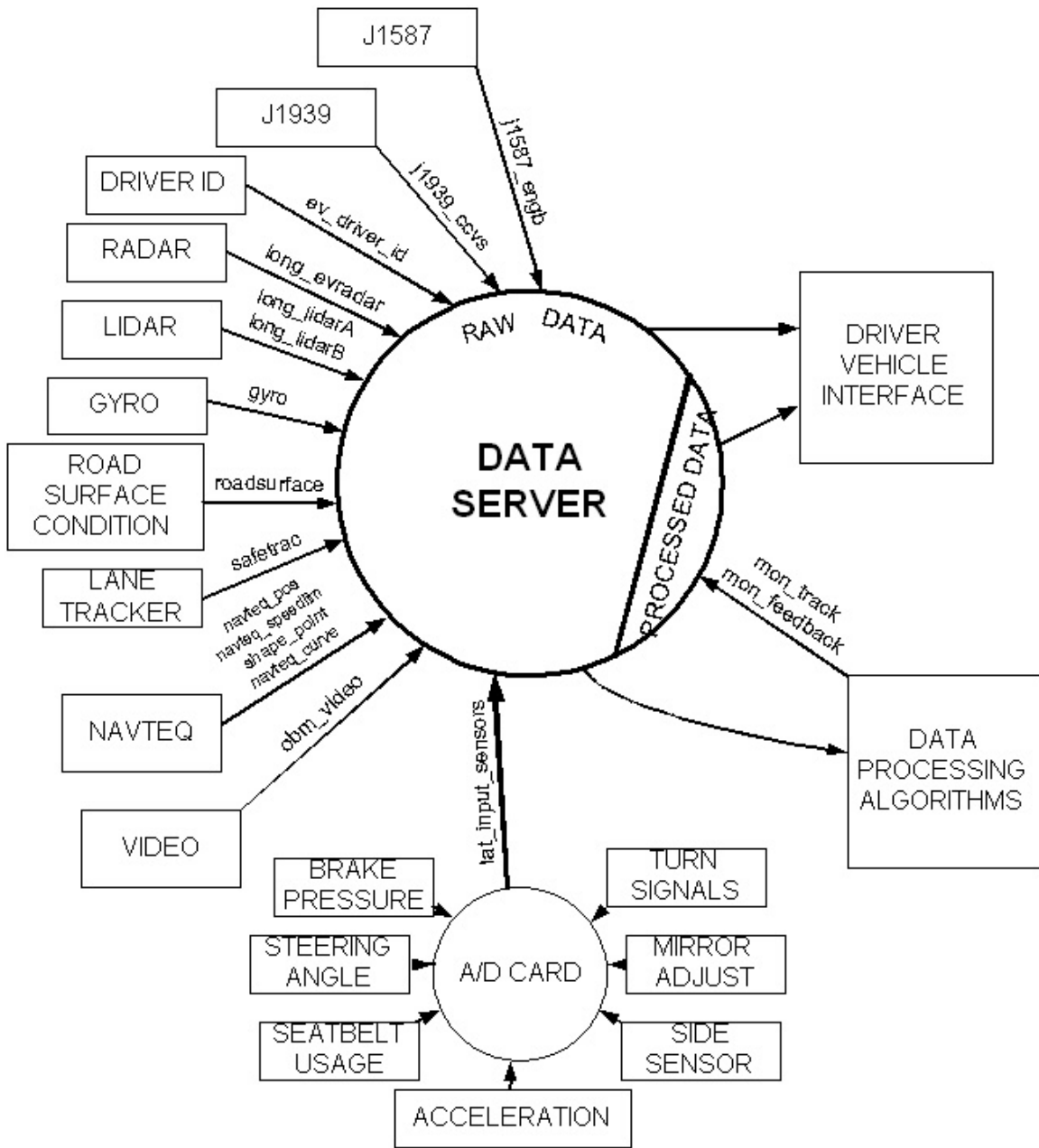
Figure 3-10. Publish and Subscribe Data Clients in OBMS Prototype
