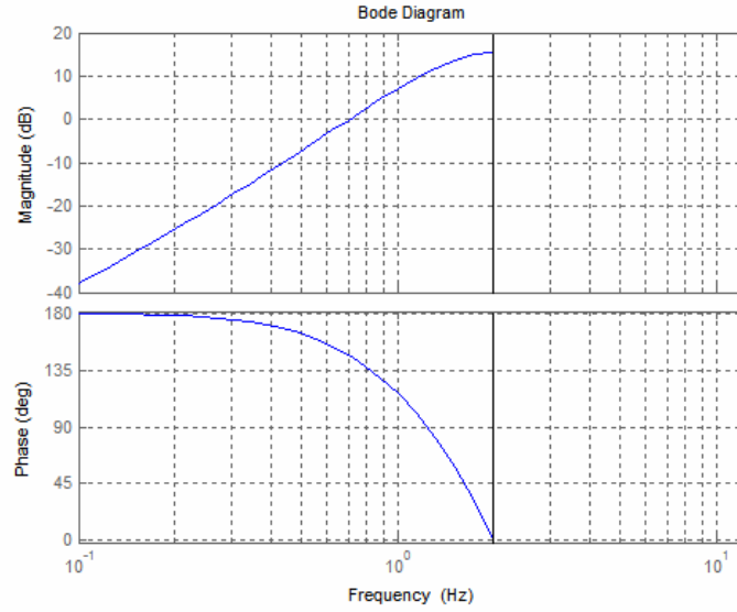
Figure 4-9. Frequency Response of the Original PE Filter with Sampling Frequency of 4Hz
