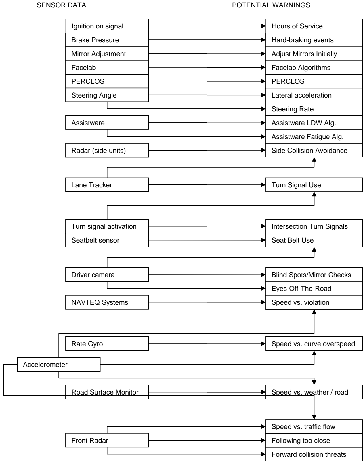
Figure A-3. Functional Relationships between Sensor Data and Monitoring System
