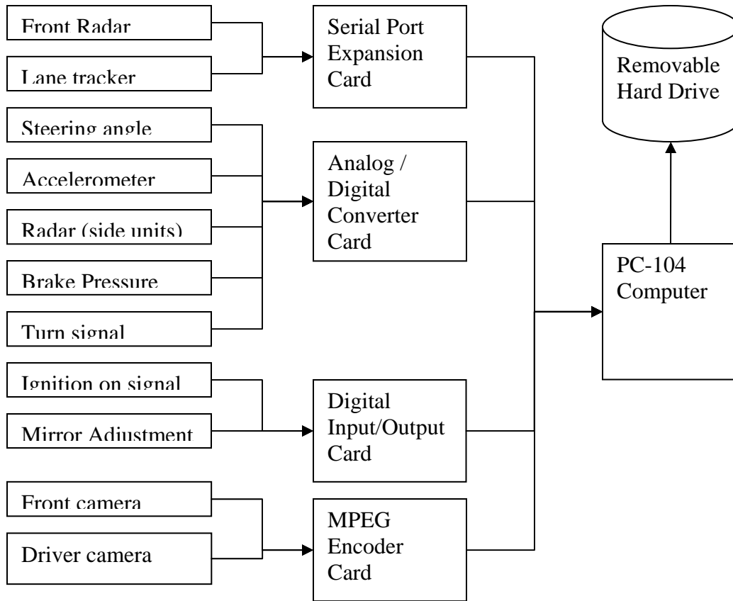
Figure A-2. Overview of Hardware Integration Components/Topics
