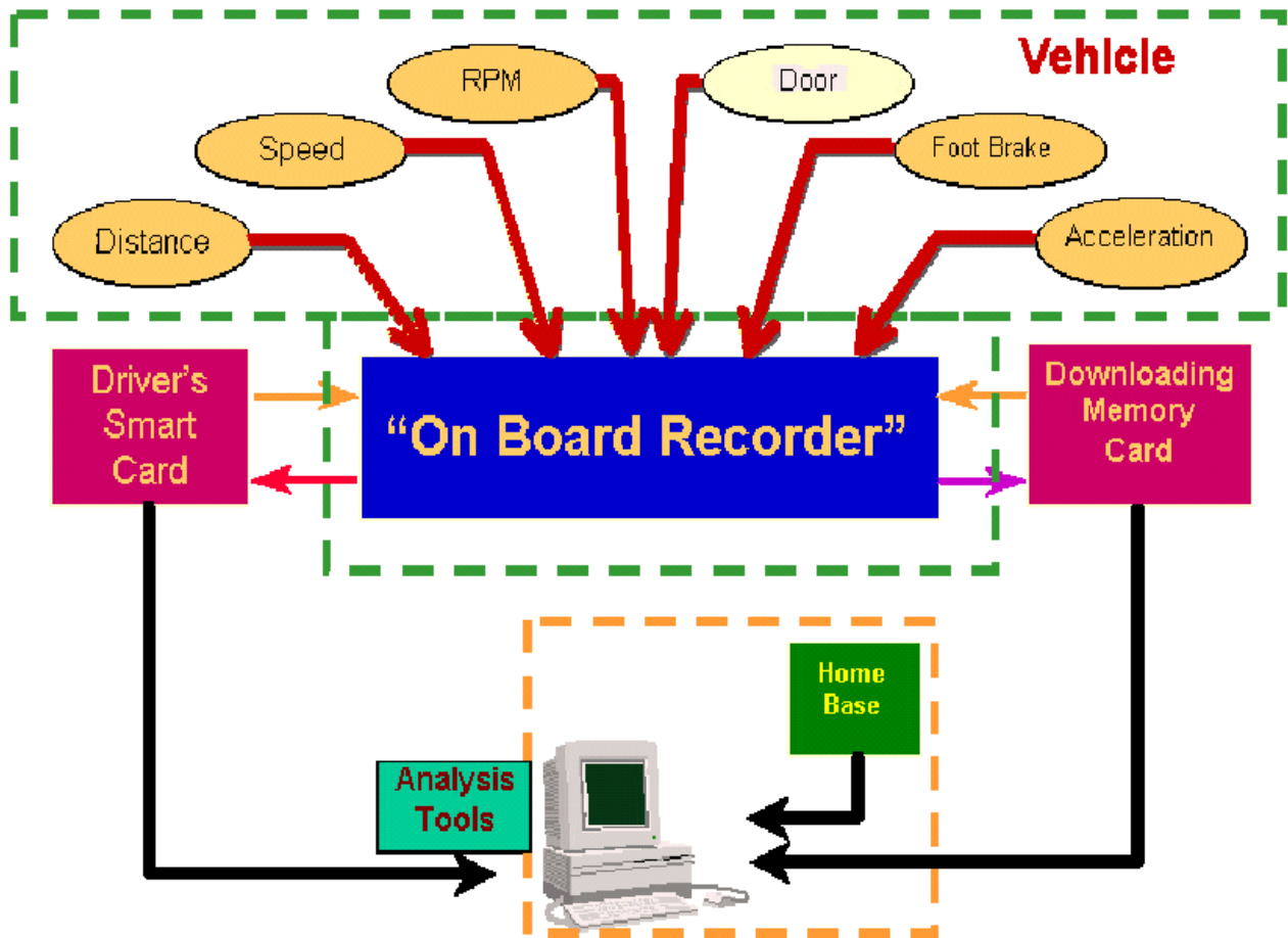
Figure 2-2. A Typical OBM System 1
