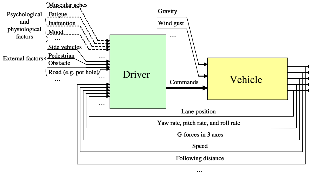
Figure 4-6. General Driver-Vehicle Interactions
