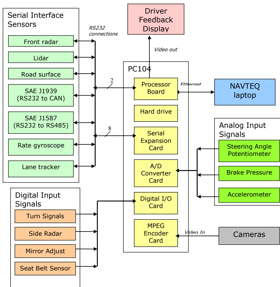
Figure 3-1. Block diagram of OBMS prototype PC104 and sensor interfaces
