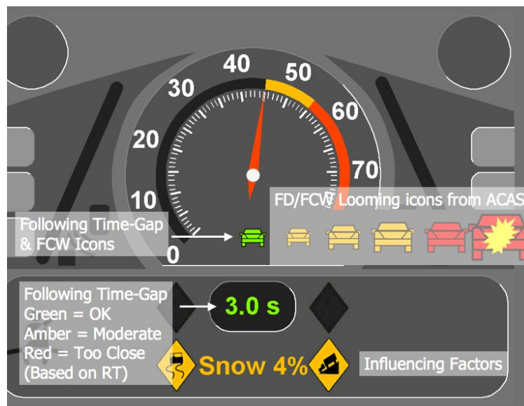
Figure 5-2. OBMS Prototype Following Time-Gap Visual Feedback Design
