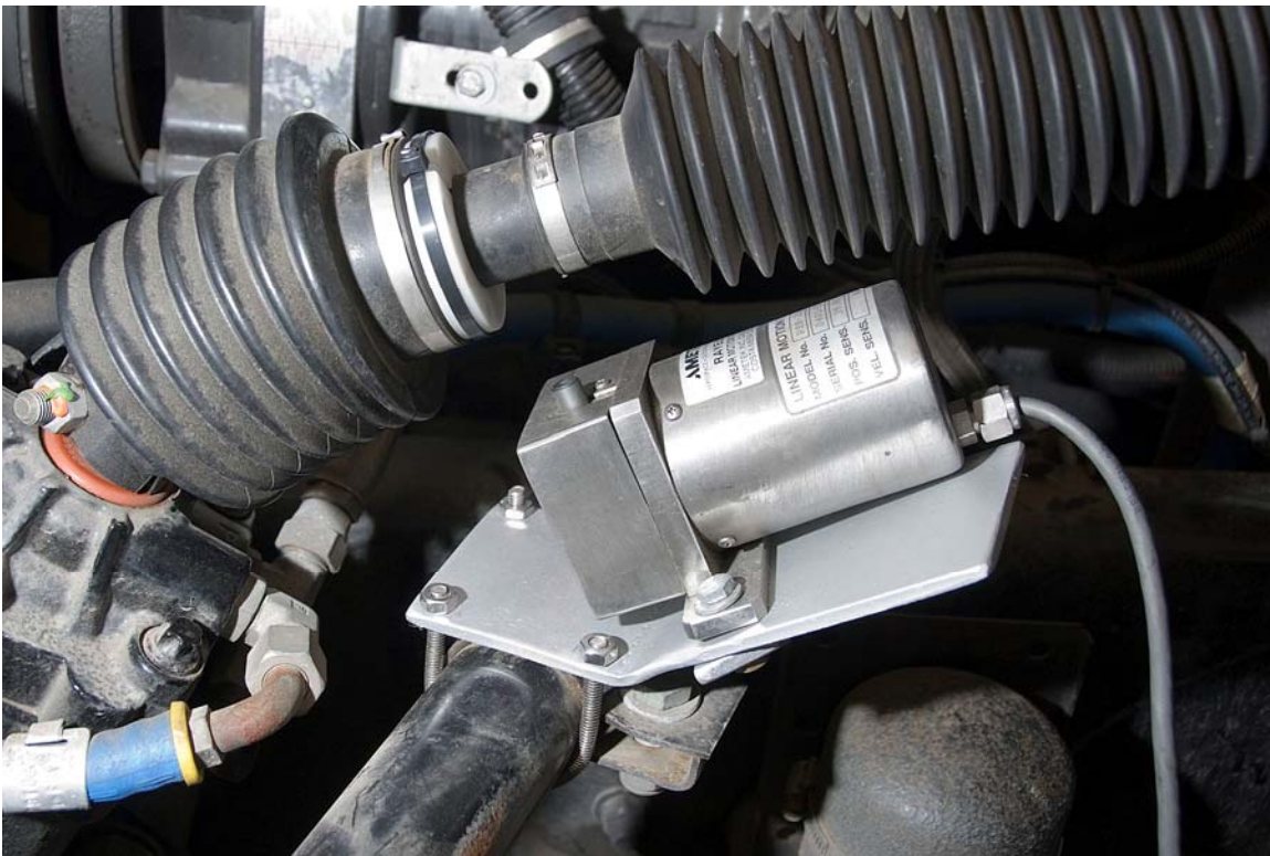
Figure 3-6. Steering Wheel Angle Sensor (String Potentiometer)
