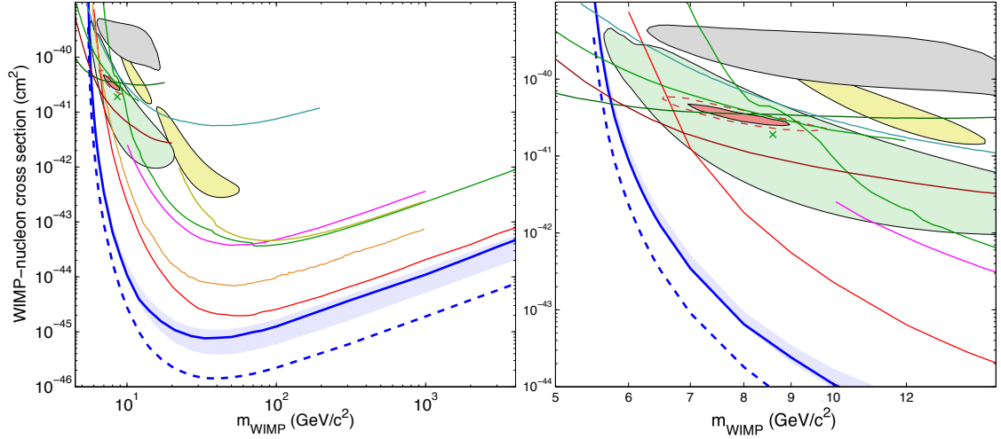
Figure 3: Left : The LUX 90% confidence limit on the spin-independent elastic WIMP-nucleon cross-section (solid blue line) and 300-day projected sensitivity (dashed blue), together with the \pm 1\sigma variation from repeated trials, where trials fluctuating below the Poisson limit from a background-free experiment recording zero counts are forced to 2.3 events (blue shaded). We also show Edelweiss II [53] (dark yellow line), CDMS II [44] (green line), ZEPLIN-III [20] (magenta line), CDMSlite [54] (dark green line), XENON10 S2-only [36] (brown line), SIMPLE [55] (light blue line), and XENON100 100 live-day [22] (orange line) and 225 live-day [21] (red line) results. Right (zoom): In addition to the LUX limit, the regions measured from annual modulation in CoGeT [45] (light red, shaded) are shown, along with exclusion limits from low threshold re-analysis of CDMS II data [56] (upper green line), 95% allowed region from CDMS II silicon detectors [51] (green shaded) and centroid (green X), 90% allowed region from CRESST II [50] (yellow shaded), and DAMA/LIBRA allowed region [49], as interpreted by [57] (gray shaded).
