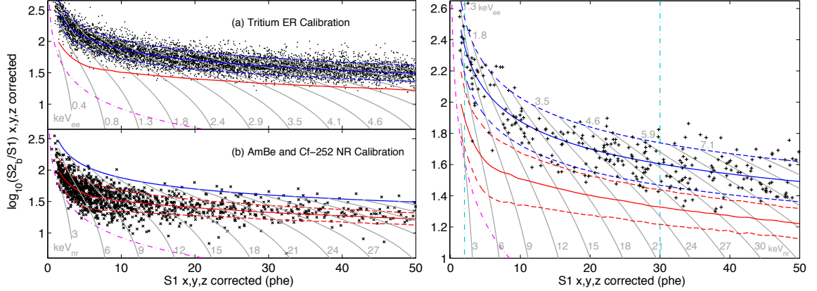
Figure 2: Left: Calibrations of detector response in the 118 kg fiducial volume. The ER (tritium, panel a ) and NR (AmBe and ^{252}\text{Cf} , panel b ) calibrations are depicted, with the means (solid line) and \pm 1.28\sigma contours (dashed lines). This choice of band width (indicating 10% band tails) is for presentation only. Panel a shows fits to the high statistics tritium data, with fits to simulated NR data shown in panel b , representing the parameterizations taken forward to the profile likelihood analysis. The ER plot also shows the NR band mean and vice versa. Gray contours indicate constant energies using an S1–S2 combined energy scale (same contours on each plot). The dot-dashed magenta line delineates the approximate location of the minimum S2 cut. Right: LUX WIMP signal region. Events in the 118 kg fiducial volume during the 85.3 live-day exposure are shown. Lines are as shown on the left, with vertical dashed cyan lines showing the 2–30 phe range used for the signal estimation analysis.
