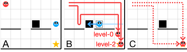
Figure 1: Example. (A) RED and BLUE in the environment at timestep t = 0 . (B) BLUE pushes the box to the left. A level-0 RED backtracks and fails, while a level-2 RED correctly infers BLUE’s intent to hinder and succeeds. (C) Some of RED’s possible counterfactual paths if BLUE hadn’t been there.
