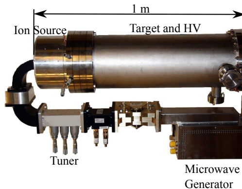
Figure 1: Neutron generator setup
