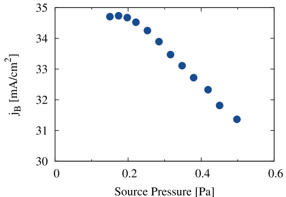
Figure 4: Dependency of beam current on pressure at 400\text{ W} microwave power.
