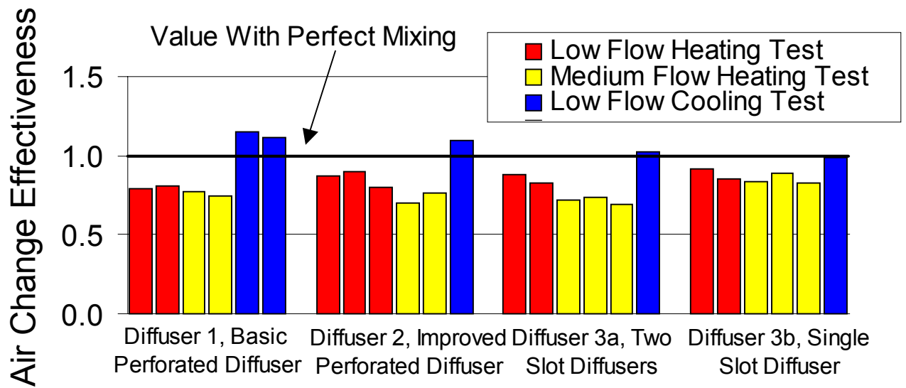
Figure 2. Measured air change effectiveness grouped by diffuser type.
