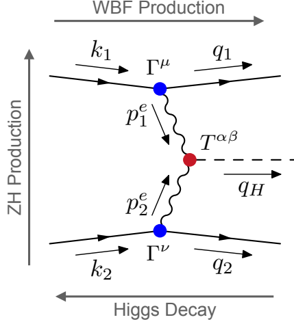
Figure 8. Feynman diagram for WBF-Higgs production, ZH production and Higgs decay to 4 leptons. The arrows indicate the momentum assignment used in the text.
