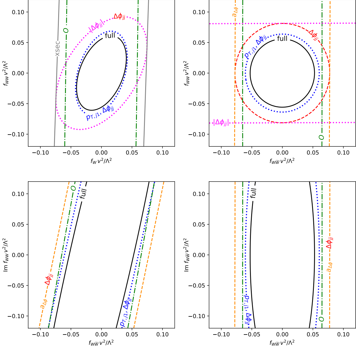
Figure 3. Optimal 1\sigma contours for WBF Higgs production with H \rightarrow \tau\tau (solid black). Also shown are the results based on different subsets of the \Delta\phi_{jj} distribution, including its absolute value (purple), its asymmetry (orange), its full distribution (red), its combination with the leading jet p_T distribution (blue); as well as the observable O as defined in Eq. (23) (green). In grey we show bounds based on a simple rate measurement. In each panel, the parameters not shown are set to zero.
