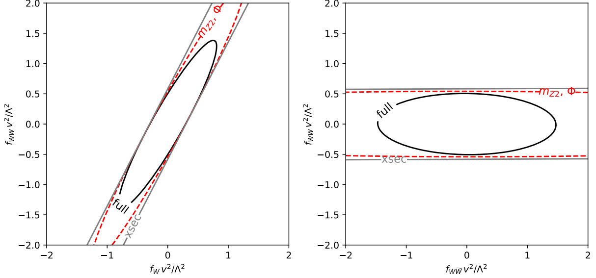
Figure 6. Optimal 1\sigma contours for gg \rightarrow h \rightarrow 4\ell (solid black). In grey we show bounds based on a rate measurement. The red line shows the contours based on an analysis of the lower of the two lepton pair masses m_{Z_2} and \Phi , other kinematic variables lead to bounds between the red and grey lines. In each panel, the parameters not shown are set to zero.
