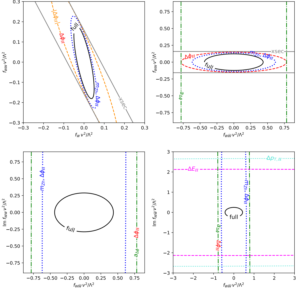
Figure 5. Optimal 1\sigma contours for ZH production (solid black). The colored lines show the reach contained in the \Delta\phi_{\ell\ell} distribution, including its absolute value (orange), asymmetry (green), full distribution (red), combination with the m_{ZH} distribution (blue); based on the distribution of \Delta E_{\ell\ell} (purple); for the distribution of \Delta p_{T,\ell\ell} (turquoise); and based on a simple rate measurement (grey). In each panel, the parameters not shown are set to zero.
