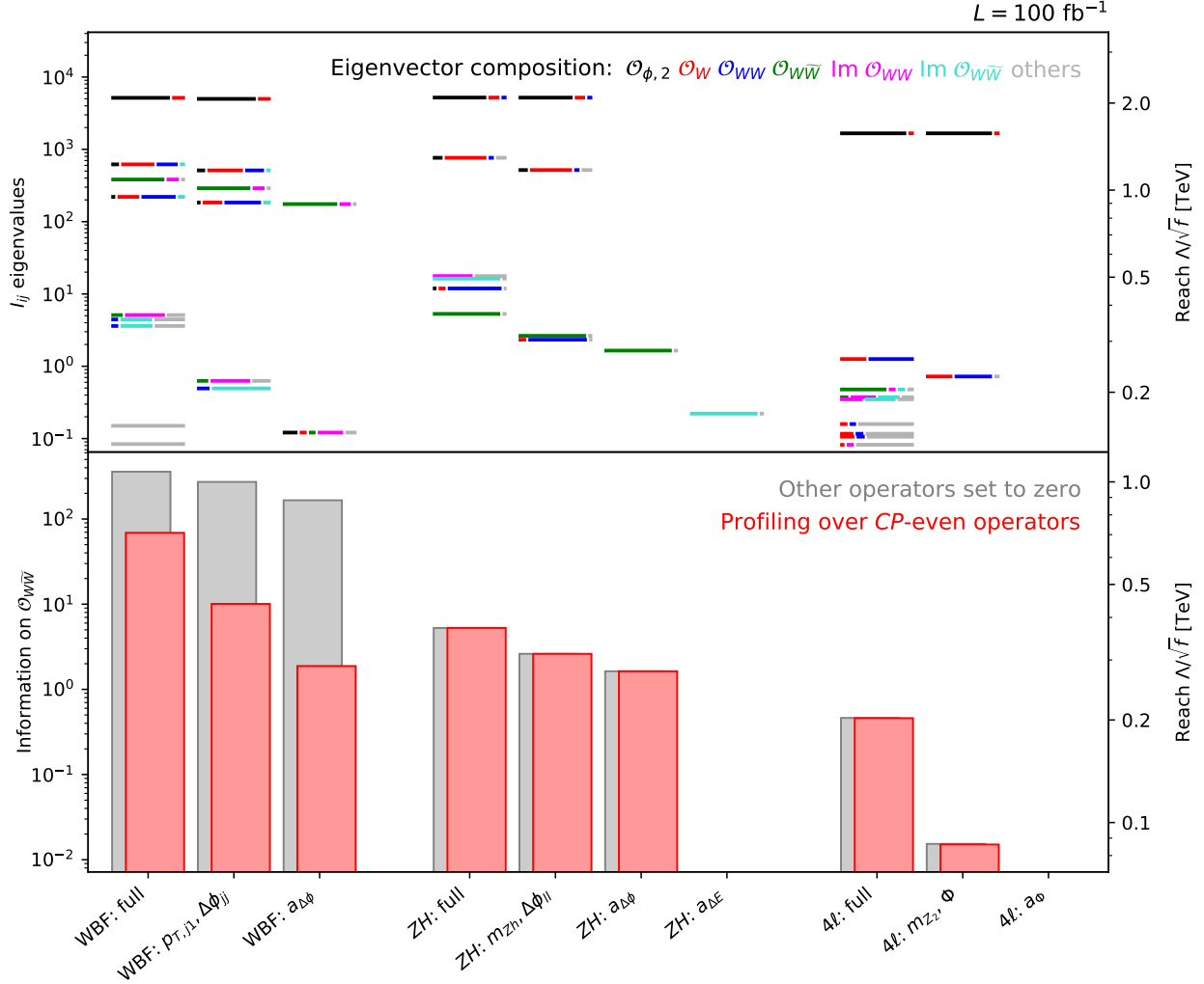
Figure 7. Comparison of the sensitivity of different channels and observables at the LHC with 100 \text{ fb}^{-1} . In the top panel we show the eigenvalues of the various Fisher information matrices. The colors denote the decomposition of the corresponding eigenvectors: the length of each segment is proportional to the magnitude of the eigenvector component. In the bottom panel we show the Fisher information on the CP -violating Wilson coefficient f_{W\bar{W}} . The grey bars show the sensitivity assuming that all other considered operators are zero, while the red bars profile over arbitrary values of all of the CP -even parameters (including absorptive parts). In both panels, the right axes translate the Fisher information into the corresponding new physics reach.
