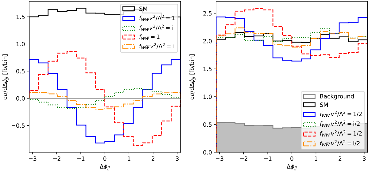
Figure 2. Distribution of the signed angle \Delta\phi_{jj} in WBF Higgs production after the cuts in Eqs. (27) and (29) for the Standard Model (black) as well as the for the EFT with the indicated Wilson coefficients. In the left panel we show the SM signal (black) as well as the interference of different dimension-six amplitudes with the SM signal (colored). The right panel shows the full distributions including the backgrounds (grey).
