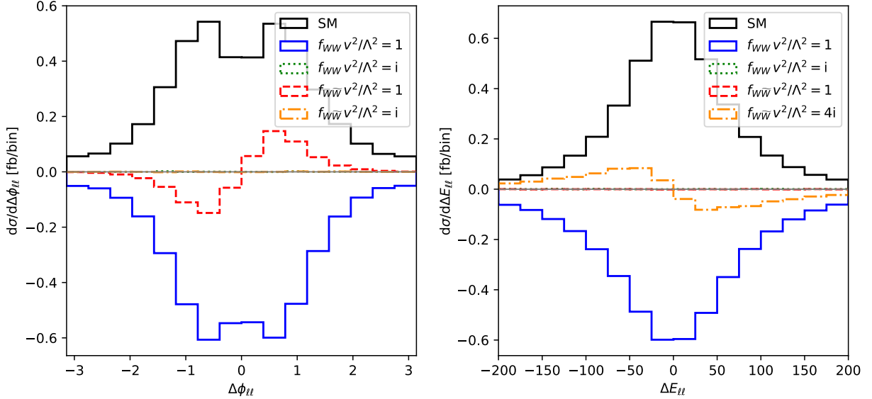
Figure 4. Distributions of \Delta\phi_{\ell\ell} (left) and \Delta E_{\ell\ell} (right) in ZH production after the cuts in Eqs. (38) and (40) for the Standard Model signal (solid black), and for the interference between different dimension-six amplitudes with the SM signal (colored).
