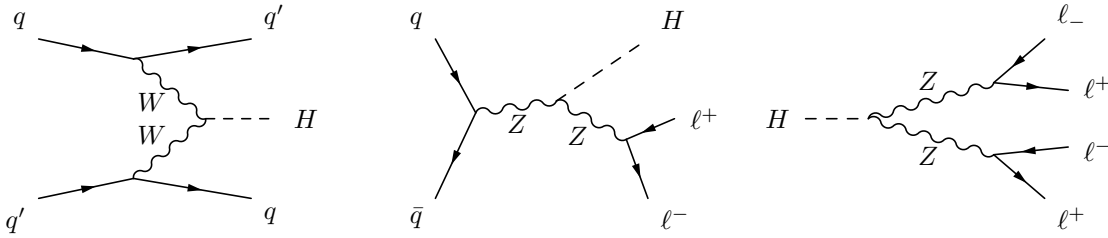
Figure 1. Feynman diagrams describing the three processes considered in this paper: WBF Higgs production, associated ZH production, and H \rightarrow 4\ell decays.
