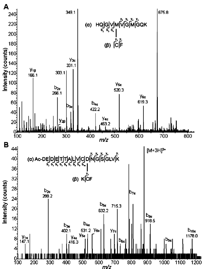
Figure 4. MS sequencing of the BPM-cross-linked actin peptides. (A) MS/MS spectrum of the [M + 3H]^{3+} of the BPM-cross-linked tryptic peptides at m/z 578.9 in the presence of cofilin. Peptides ( \alpha ) and ( \beta ) are from the same G-actin. Singly and doubly charged y -type product ions were generated from dissociation of the 3+-charged precursor ion. (Peptide fragments are denoted following the nomenclature for fragmentation of cross-linked oligopeptides. Subscripts are used to denote the residue position, counting from the N terminus for a_n , b_n , and c_n ions and from the C terminus for x_n , y_n , and z_n products.) (B) MS/MS spectrum of the [M + 3H]^{3+} of the BPM-cross-linked tryptic peptides at m/z 880.4 in the absence of cofilin. The representation is the same as in (A).
