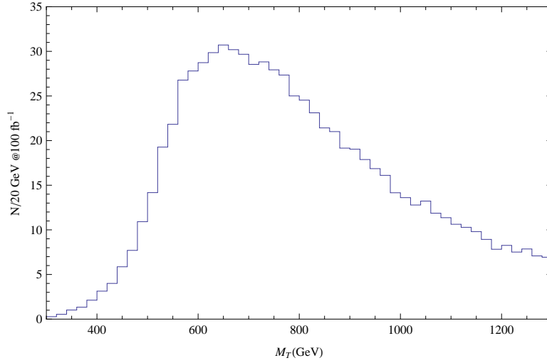
FIG. 11: The SM background for the single production channel, pp \rightarrow WZjj \rightarrow jjll , calculated by summing over the u , d , c , s and gluon jets and the first two families of leptons. The bin size is 20 GeV.
