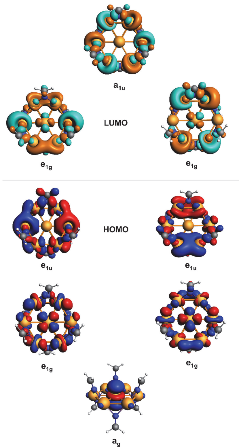
Figure 4. Frontier MOs (isosurface plots \pm 0.03 au) in Pd 7 (N=CH 2 ) 6 (a truncated model complex of 1 ).
