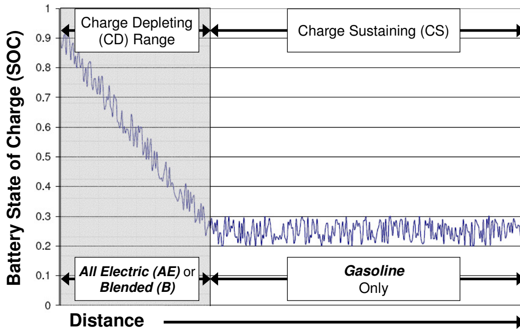
Fig. 1: Illustration of typical PHEV discharge cycle (~65% depth of discharge)
