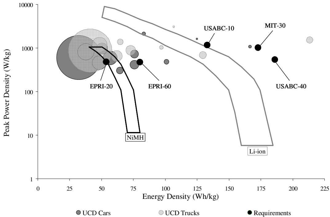
Fig. 2: Distribution of battery requirements for PHEV designs selected by potential early market respondents and USABC, MIT, and EPRI
