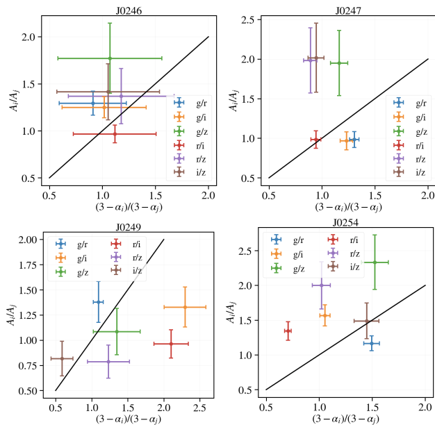
Figure 4. Observed frequency-dependent variability amplitude ratios compared with the expected values from the Doppler boost model. Different colors represent different combinations of band pairs. The black lines represent the 1 to 1 relation. Error bars denote 1\sigma uncertainties. See §5.2 for details.
