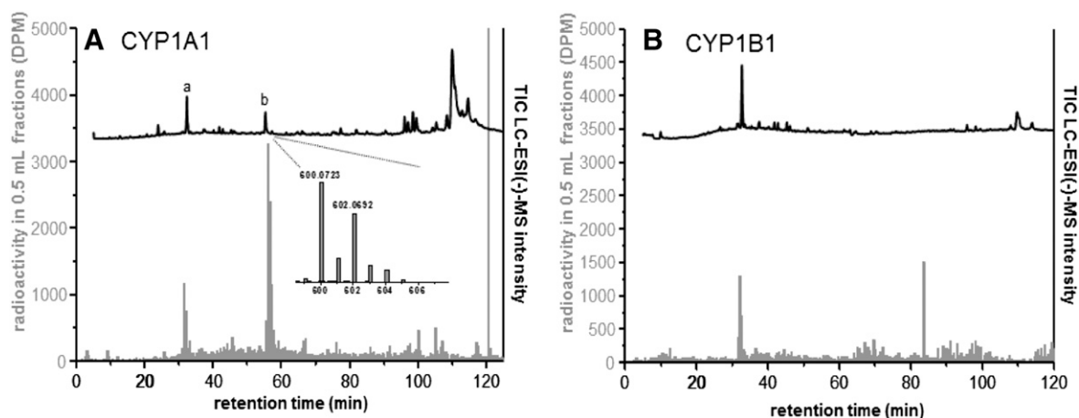
Fig. 1. Radioactivity profile of LC fractions and LC-ESI(-)-MS chromatograms of incubation of TCC with CYP1A1 (A) and CYP1B1 (B). Inset: MS spectrum of the peak eluting at 55.3 minutes.
