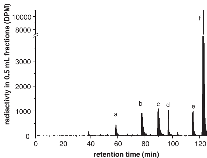
Fig. 4. Radioactivity profile of LC fractions after incubation of TCDD-induced keratinocytes with TCC for 24 hours. The peaks correspond to DHC-GSH adduct (a), DHC (b), 2-O-Gluc TCC (c), 3'-OH-TCC (d), 2' OH-TCC and 6 OH-TCC (e), and TCC (f).
