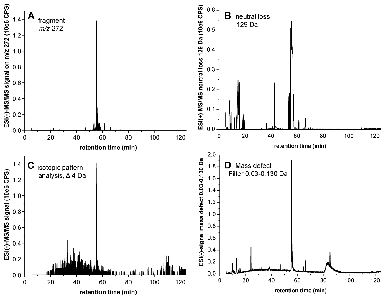
Fig. 2. Extracted ion signals for diagnostic fragments of GSH adducts of incubation of TCC with CYP1A1. (A) ESI(-)-MS/MS of the GSH fragment at m/z 272 and (B) ESI(+)-MS/MS neutral loss scan of 129 Da. (C) Isotopic pattern analysis for two chlorine atoms. (D) Mass defect analysis for the DHC-GSH adduct.
