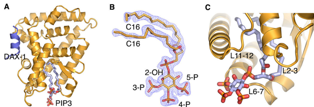
Figure 2. Structure of PIP 3 bound LRH-1
