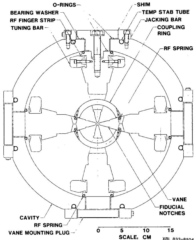
Figure 1: Typical cross section of RFQ
