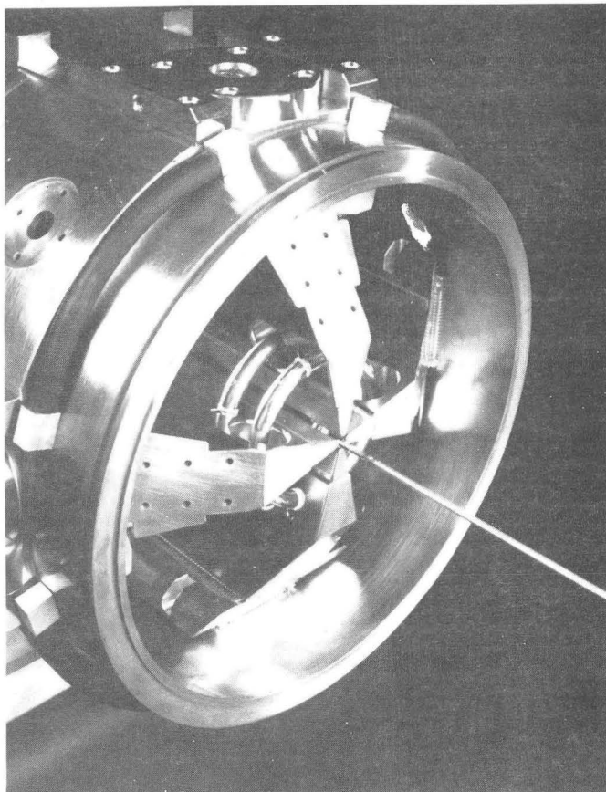
Figure 4: Measuring aperture between vane tips
