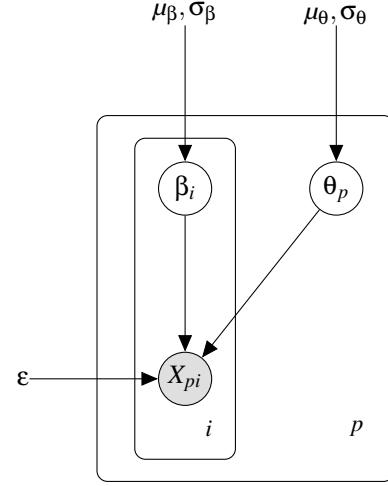
Figure 1: Graphical representation of the model: each observed response X_{pi} is influenced by latent variables \beta_i (drawn from the difficulty prior) and \theta_p (perceived ability prior) as well as a constant \epsilon (likelihood). \beta_i is drawn from a normal distribution with mean \mu_\beta and standard deviation \sigma_\beta and \theta_p is normal with mean \mu_\theta and standard deviation \sigma_\theta .
