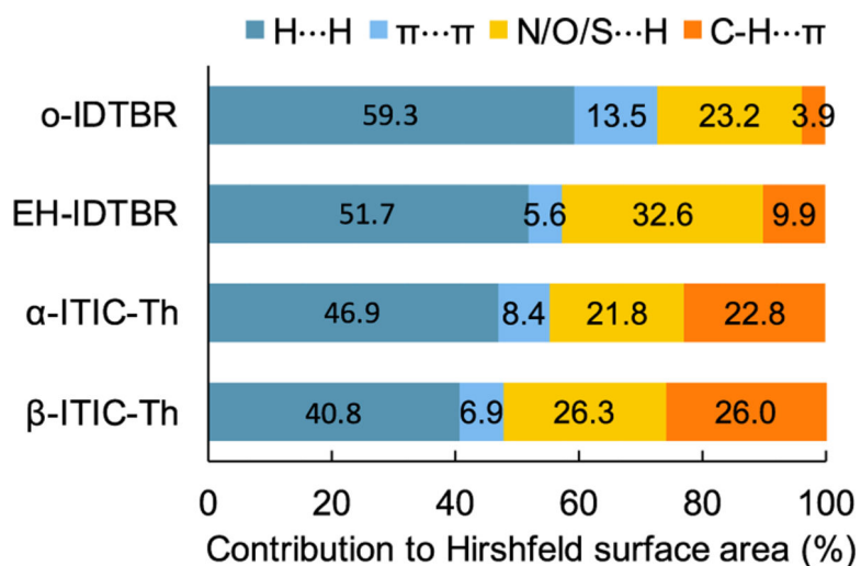
Figure 7. Comparison of Hirshfeld surface contributions for o-IDTBR, EH-IDTBR, \alpha -ITIC-Th, and \beta -ITIC-Th. Comparison of four different types of interactions (H...H contacts, C-H... \pi interactions, \pi ... \pi stacking, and N/O/S...H contacts) to the area of the Hirshfeld surface enables quantitative analysis of the contributions of intermolecular forces to the MicroED structures. The Hirshfeld surface analysis does not directly quantify C-H... \pi interactions or \pi ... \pi stacking. H...C contacts were used to approximate the C-H... \pi interactions, and C...C, C...X (X = N, O, S), and X...X contacts were used to approximate the \pi ... \pi stacking. Full details are given in the Methods section.
