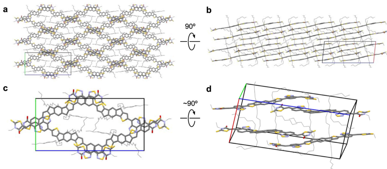
Figure 2. Lattice of o-IDTBR determined from MicroED. Views of the o-IDTBR MicroED structure along the a -axis (a) and the b -axis (b) of the unit cell. View of four o-IDTBR molecules that form a parallelogram in the 3D wire mesh (c). Side view of the same parallelogram to emphasize the lack of direct contact between molecules at an acute angle (d). Hydrogens are omitted for clarity, and alkyl chains are depicted as wireframe structures. The red, green, and blue axes correspond to the a , b , and c axes of the unit cell, respectively. The arrows represent a 90° rotation of the crystal around the given axis.
