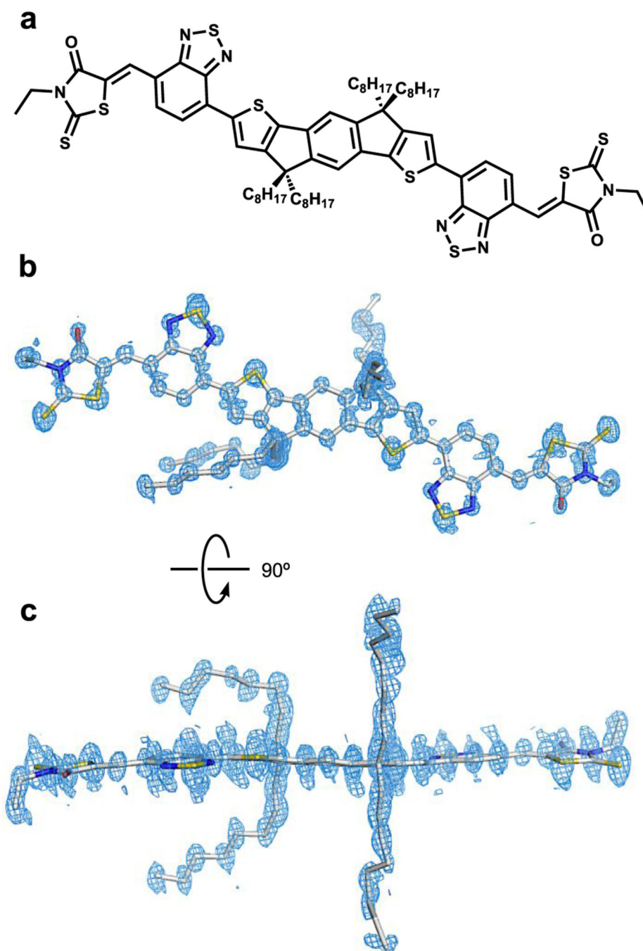
Figure 1. Molecular and MicroED structures of o-IDTBR. Molecular structure of o-IDTBR (a) and density maps and 0.9 Å resolution structure of o-IDTBR determined by MicroED as viewed normal to the plane of the backbone (b) and in the plane of the backbone (c) to highlight the orthogonal arrangement of the octyl chains. Maps are 2mF_o - dF_c maps contoured at the 1.5\sigma level with a 2 Å carve for clarity. The arrow represents the 90° rotation of the crystal around the given axis.
