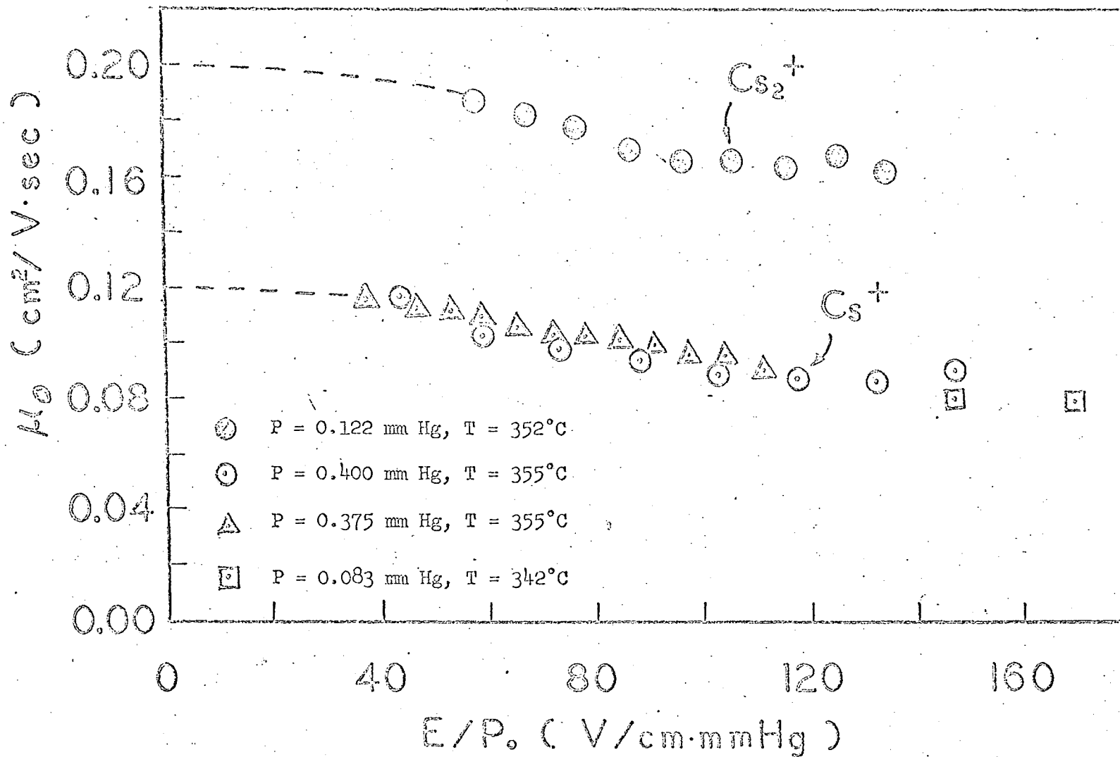
Fig. V-5. The variation of the normalized mobilities of \text{Cs}^+ and \text{Cs}_2^+ with E/P_0
