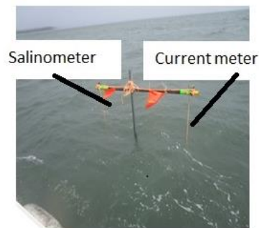
Figure 4: Observations for Salinity and flow velocity during from 14 July to 14 September in 2015. The water depth is about 130cm.
