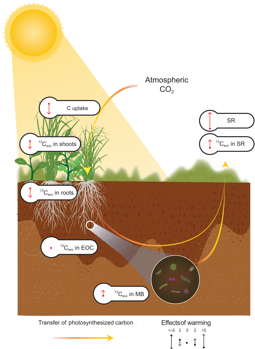
FIGURE 6 Graphical summary of the effects of 10 years of soil warming on the transfer of C from net CO 2 uptake to soil respiration (SR). The warming effect sizes on excess 13 C ( 13 C exc ) in shoot, root, soil extractable organic carbon (EOC), microbial biomass (MB) and SR are standardized regression coefficients obtained from linear mixed effects models. The upward and downward pointing arrows represent increasing and decreasing effects of warming, respectively.
