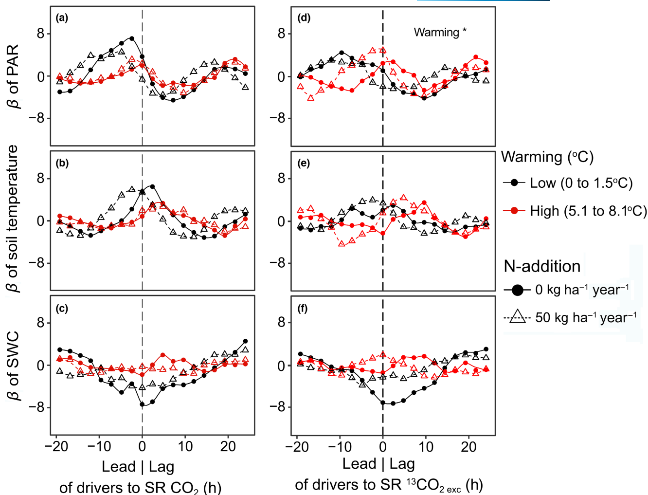
FIGURE 5 Cross correlation analysis of soil-respired \text{CO}_2 (total and ^{13}\text{CO}_2 from pulse labelling) and its environmental drivers under warming and N-addition. The standardized regression coefficients of photosynthetically active radiation (PAR) (a, d), soil temperature (b, e) and soil water content (SWC; c, f) show the relationship of the drivers with soil-respired \text{CO}_2 and excess ^{13}\text{CO}_2 ( ^{13}\text{CO}_{2\text{exc}} ) in dependence of time lags between soil respiration (SR) and drivers. Negative values on the x-axis indicate that driver fluctuations preceded fluctuations in SR and that therefore the drivers lead SR. Positive values indicate the opposite. Circles and triangles indicate measurements from unfertilized and fertilized (N-addition) plots, respectively.
