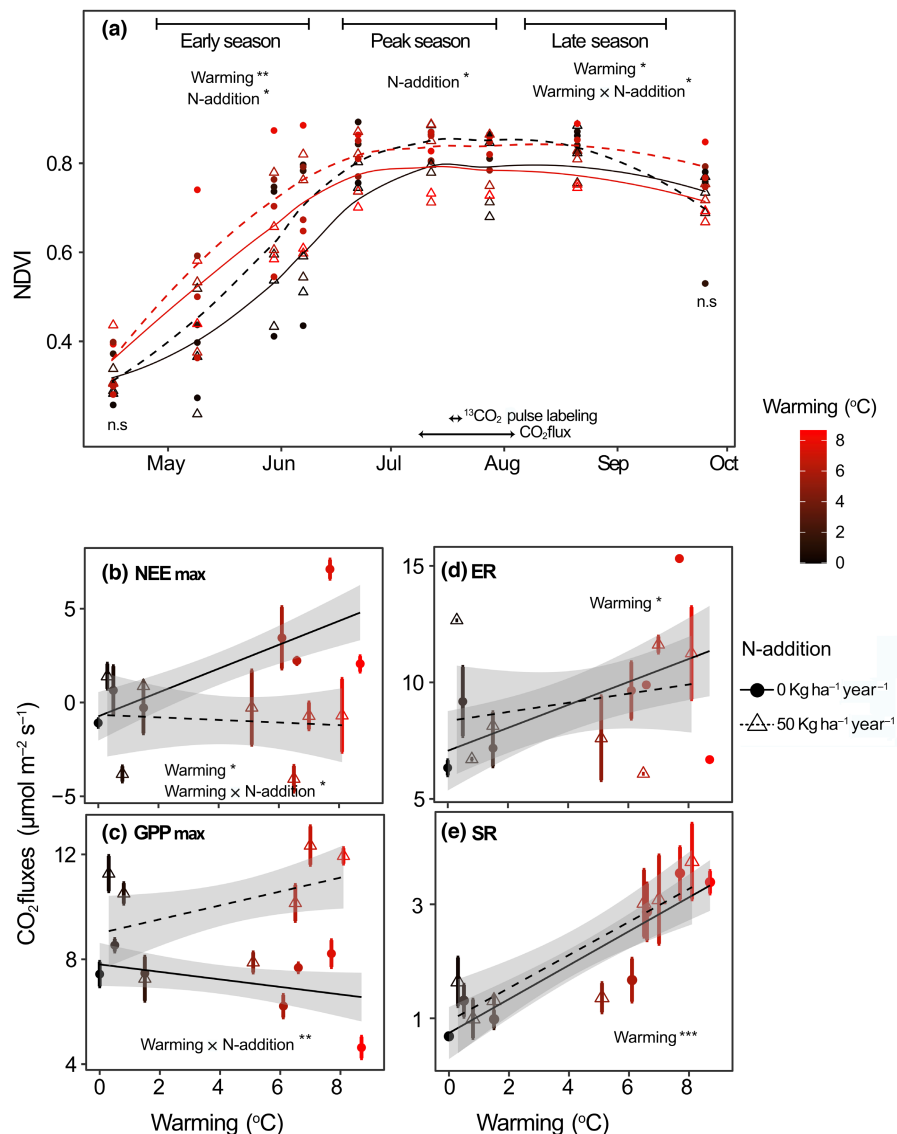
FIGURE 1 Normalized difference vegetation index (NDVI) and ecosystem \text{CO}_2 fluxes in response to warming and N addition. (a) NDVI measured during the early, peak, and late growing season. (b) Light saturated ( \text{PAR} > 1000 \mu\text{mol m}^{-2} \text{s}^{-1} ) net ecosystem exchange of \text{CO}_2 ( \text{NEE}_{\text{max}} ) and (c) gross primary productivity ( \text{GPP}_{\text{max}} ), (d) ecosystem respiration (ER) and (e) soil respiration (SR) measured along the soil warming gradient in July 2018. The ambient soil temperature of the unwarmed plots during the field campaign was 10.2^\circ\text{C} . Circles and triangles indicate measurements from unfertilized and fertilized (N-addition) plots, respectively. Error bars indicate standard errors of the mean. Asterisks denote significant effects of warming, N-addition and their interaction ( p value: <.05^* ; <.01^{**} ; <.001^{***} ).
